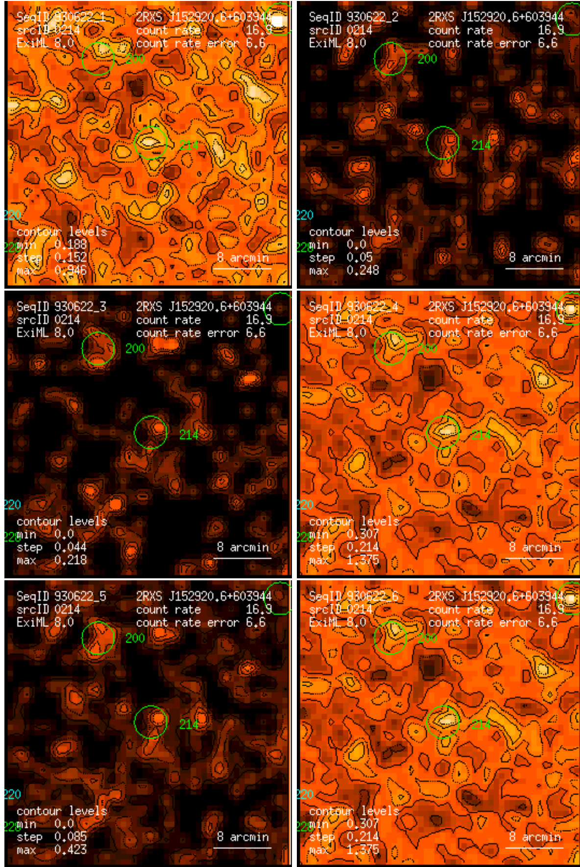
Figure 214: RASS 930622: detection 0214: band rate images, Gaussian filter: (1) PSPC channels 11 – 41, (2) 52 – 90, (3) 91 – 201, (4) 11 – 235, (5) 52 – 201, (6) 11 – 201. Broad band rates in counts/ks. Band rate contour levels in counts/ks/arcmin 2 .
