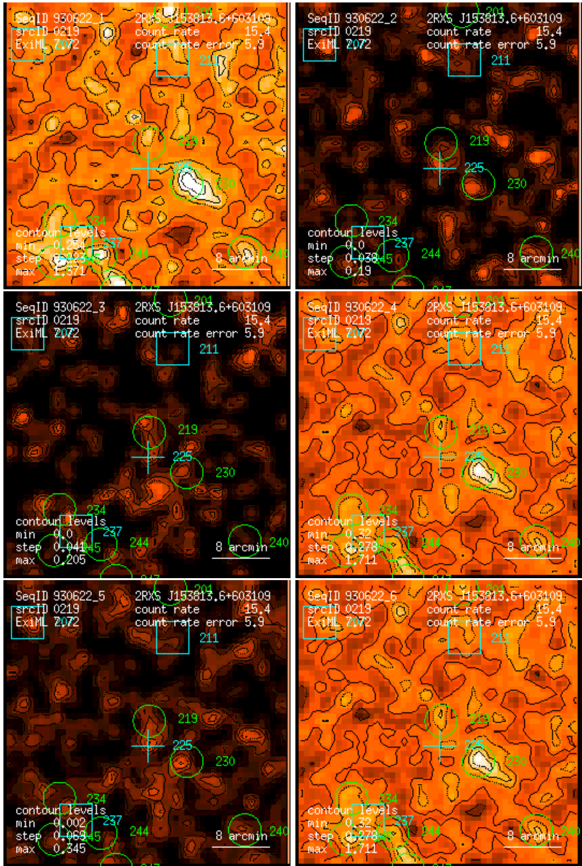
Figure 219: RASS 930622: detection 0219: band rate images, Gaussian filter: (1) PSPC channels 11 – 41, (2) 52 – 90, (3) 91 – 201, (4) 11 – 235, (5) 52 – 201, (6) 11 – 201. Broad band rates in counts/ks. Band rate contour levels in counts/ks/arcmin 2 .
