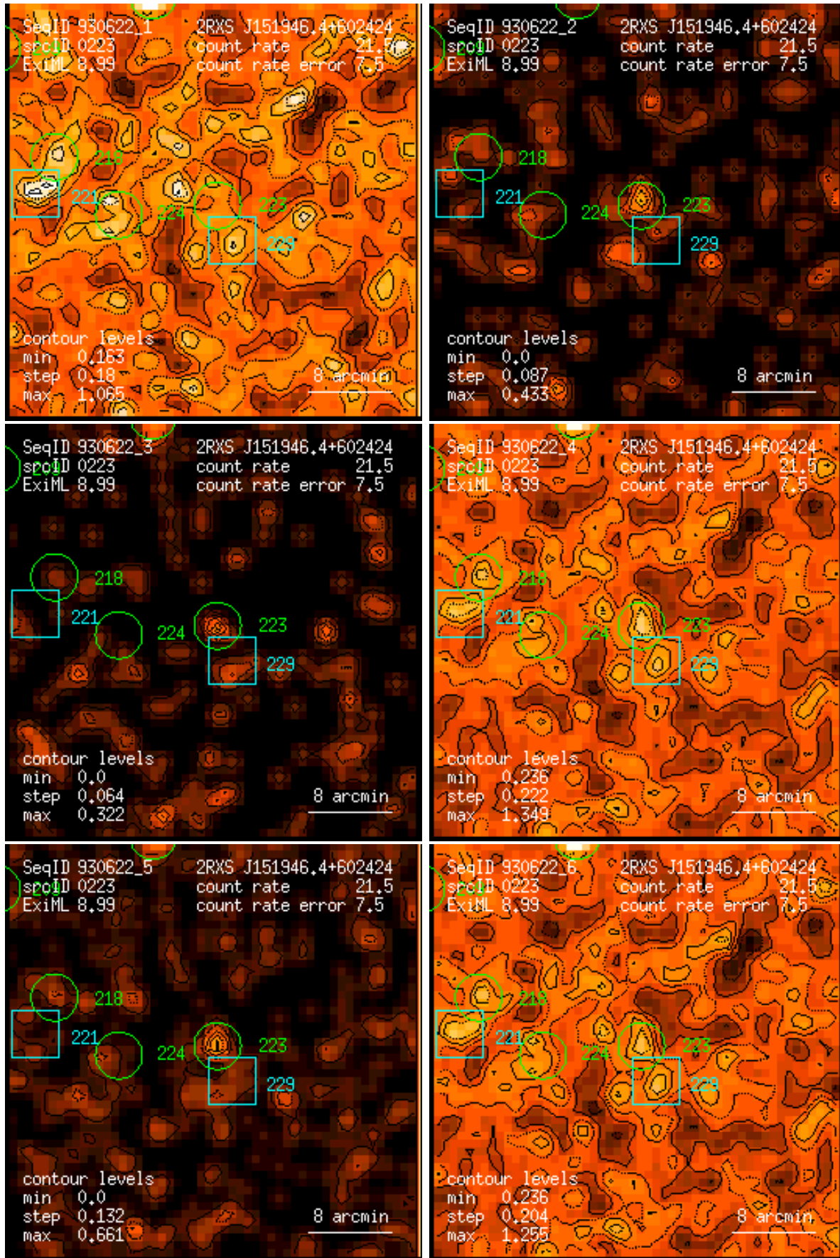
Figure 223: RASS 930622: detection 0223: band rate images, Gaussian filter: (1) PSPC channels 11 – 41, (2) 52 – 90, (3) 91 – 201, (4) 11 – 235, (5) 52 – 201, (6) 11 – 201. Broad band rates in counts/ks. Band rate contour levels in counts/ks/arcmin 2 .
