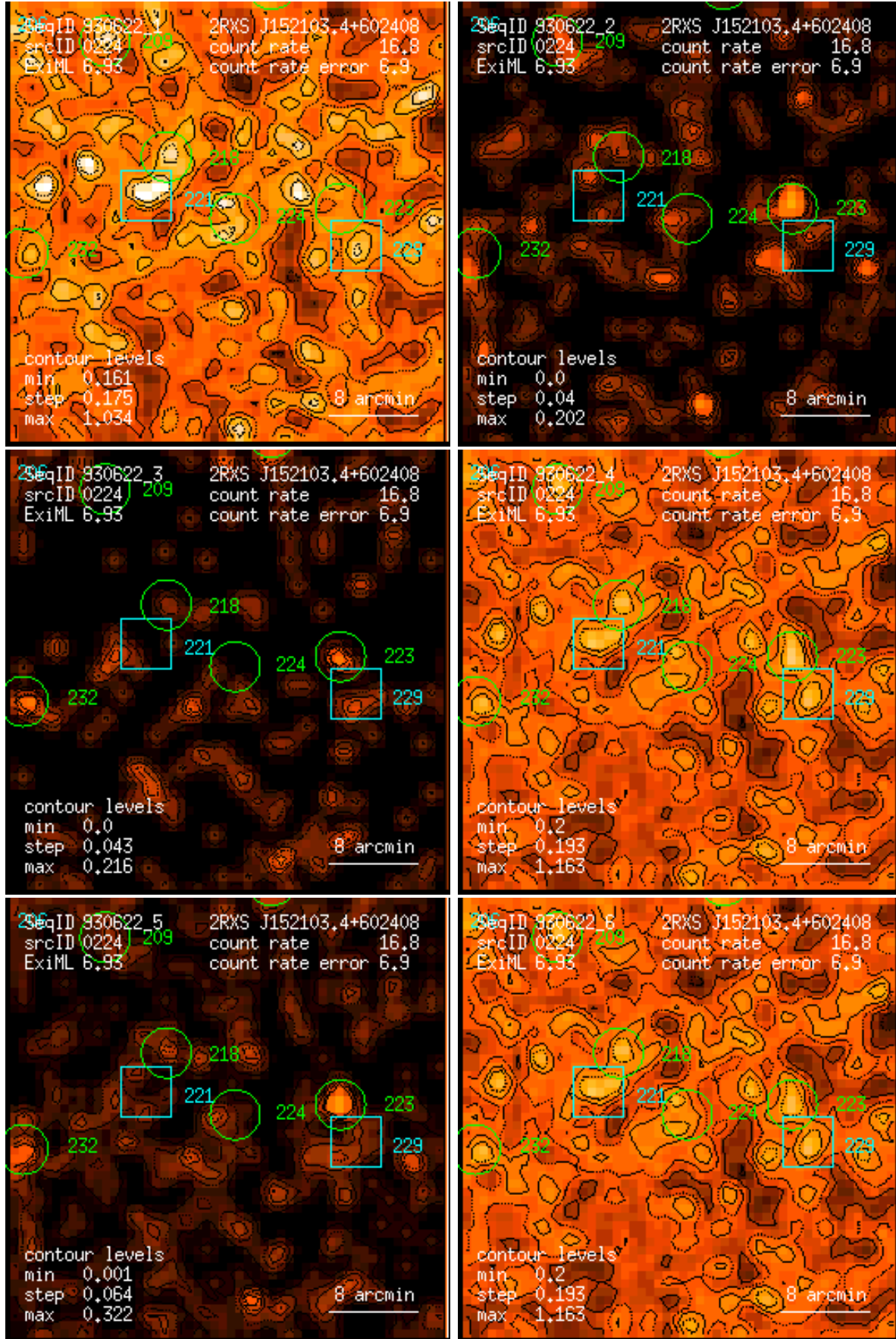
Figure 224: RASS 930622: detection 0224: band rate images, Gaussian filter: (1) PSPC channels 11 – 41, (2) 52 – 90, (3) 91 – 201, (4) 11 – 235, (5) 52 – 201, (6) 11 – 201. Broad band rates in counts/ks. Band rate contour levels in counts/ks/arcmin 2 .
