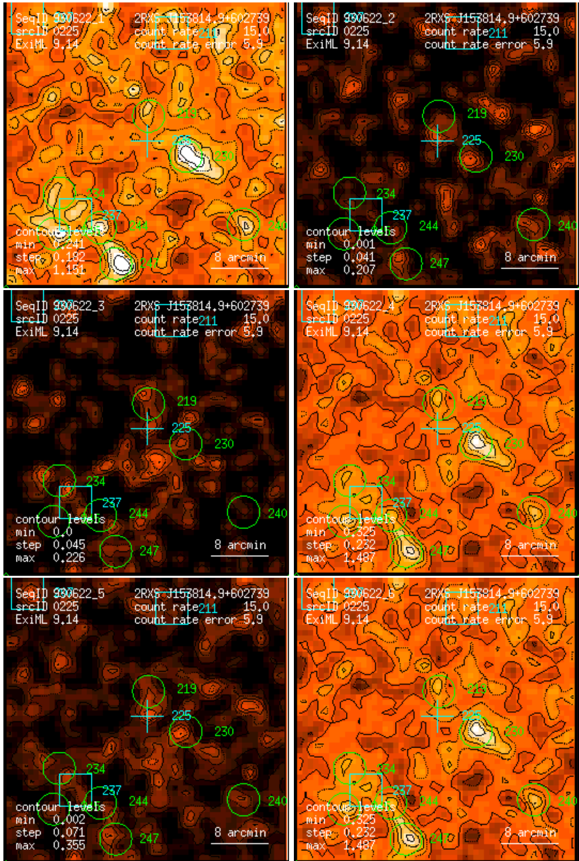
Figure 225: RASS 930622: detection 0225: band rate images, Gaussian filter: (1) PSPC channels 11 – 41, (2) 52 – 90, (3) 91 – 201, (4) 11 – 235, (5) 52 – 201, (6) 11 – 201. Broad band rates in counts/ks. Band rate contour levels in counts/ks/arcmin 2 .
