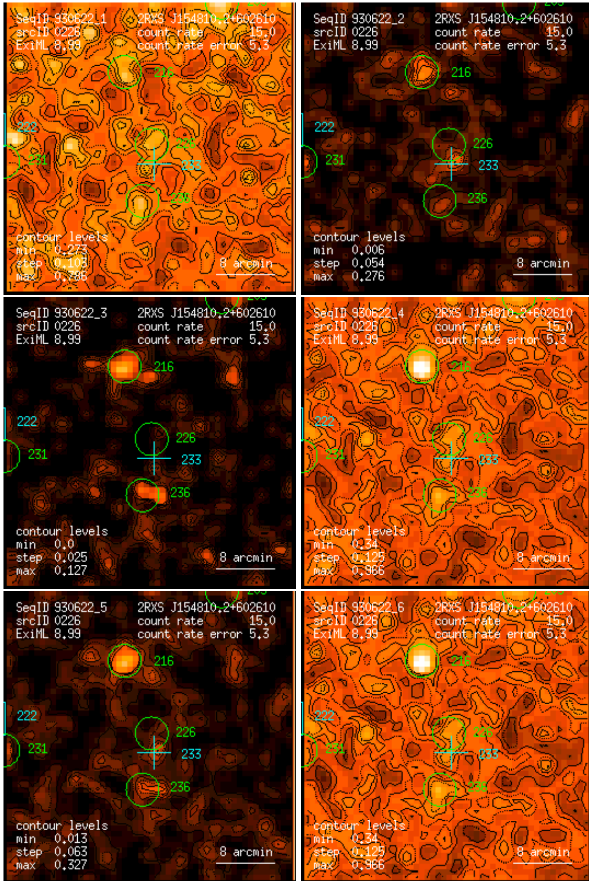
Figure 226: RASS 930622: detection 0226: band rate images, Gaussian filter: (1) PSPC channels 11 – 41, (2) 52 – 90, (3) 91 – 201, (4) 11 – 235, (5) 52 – 201, (6) 11 – 201. Broad band rates in counts/ks. Band rate contour levels in counts/ks/arcmin 2 .
