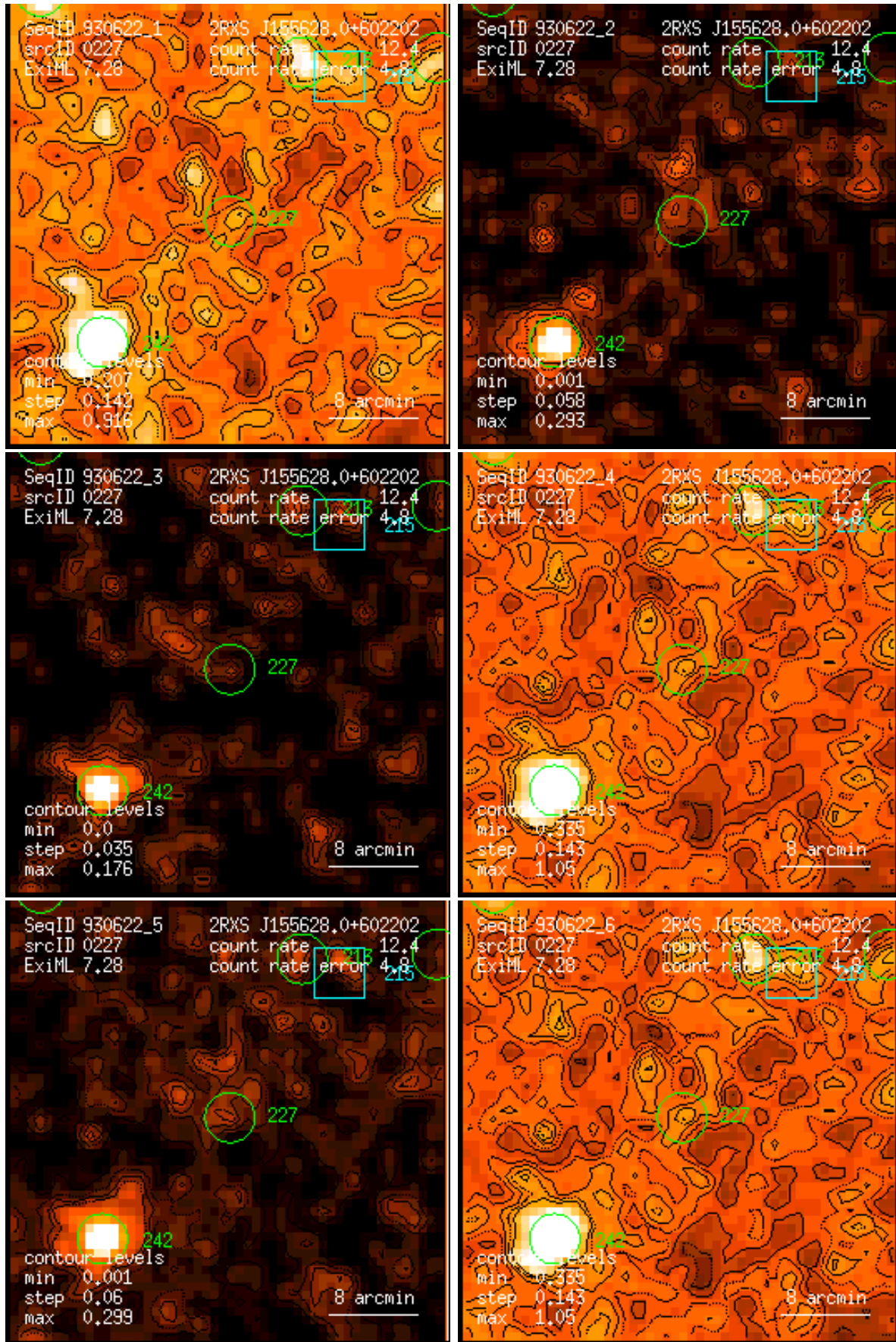
Figure 227: RASS 930622: detection 0227: band rate images, Gaussian filter: (1) PSPC channels 11 – 41, (2) 52 – 90, (3) 91 – 201, (4) 11 – 235, (5) 52 – 201, (6) 11 – 201. Broad band rates in counts/ks. Band rate contour levels in counts/ks/arcmin 2 .
