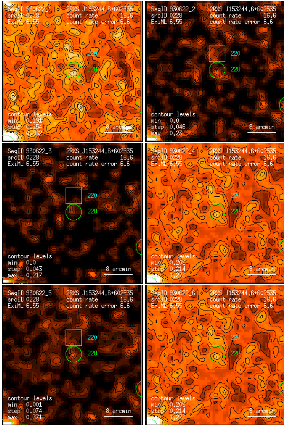
Figure 228: RASS 930622: detection 0228: band rate images, Gaussian filter: (1) PSPC channels 11 – 41, (2) 52 – 90, (3) 91 – 201, (4) 11 – 235, (5) 52 – 201, (6) 11 – 201. Broad band rates in counts/ks. Band rate contour levels in counts/ks/arcmin 2 .
