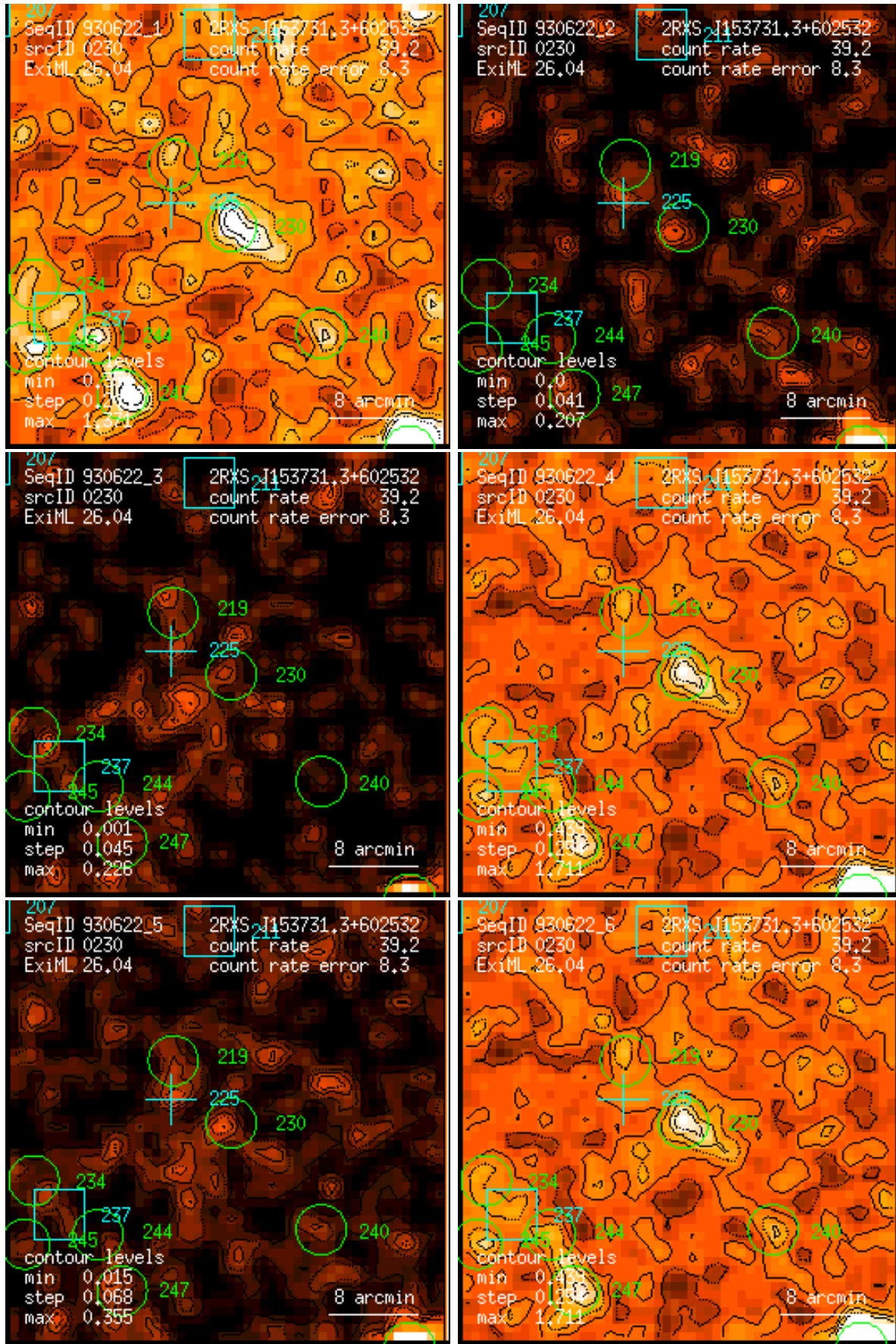
Figure 230: RASS 930622: detection 0230: band rate images, Gaussian filter: (1) PSPC channels 11 – 41, (2) 52 – 90, (3) 91 – 201, (4) 11 – 235, (5) 52 – 201, (6) 11 – 201. Broad band rates in counts/ks. Band rate contour levels in counts/ks/arcmin 2 .
