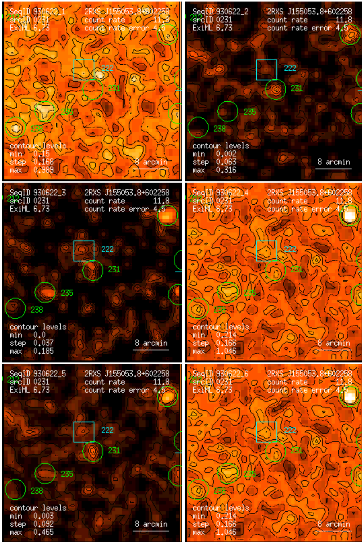
Figure 231: RASS 930622: detection 0231: band rate images, Gaussian filter: (1) PSPC channels 11 – 41, (2) 52 – 90, (3) 91 – 201, (4) 11 – 235, (5) 52 – 201, (6) 11 – 201. Broad band rates in counts/ks. Band rate contour levels in counts/ks/arcmin 2 .
