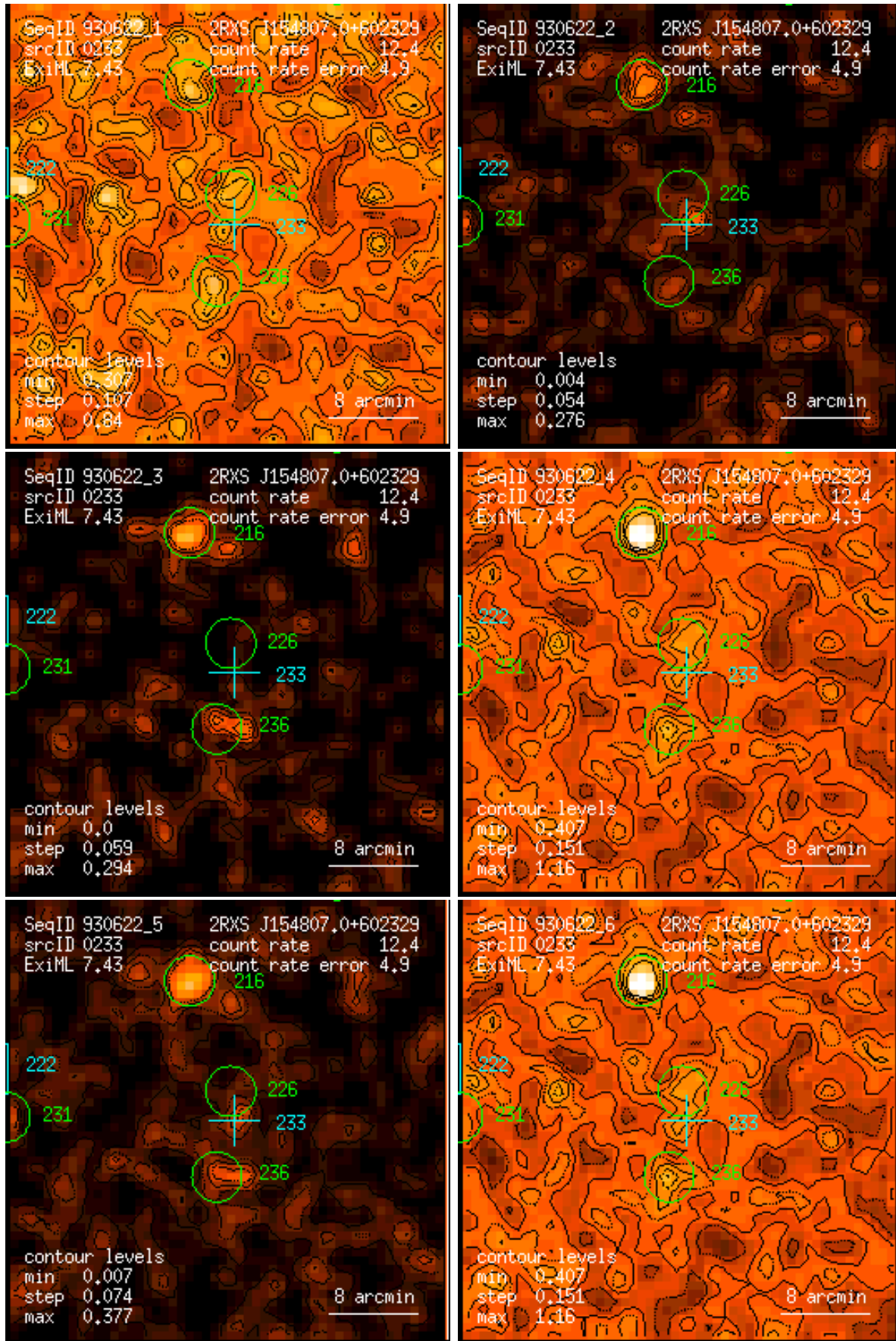
Figure 233: RASS 930622: detection 0233: band rate images, Gaussian filter: (1) PSPC channels 11 – 41, (2) 52 – 90, (3) 91 – 201, (4) 11 – 235, (5) 52 – 201, (6) 11 – 201. Broad band rates in counts/ks. Band rate contour levels in counts/ks/arcmin 2 .
