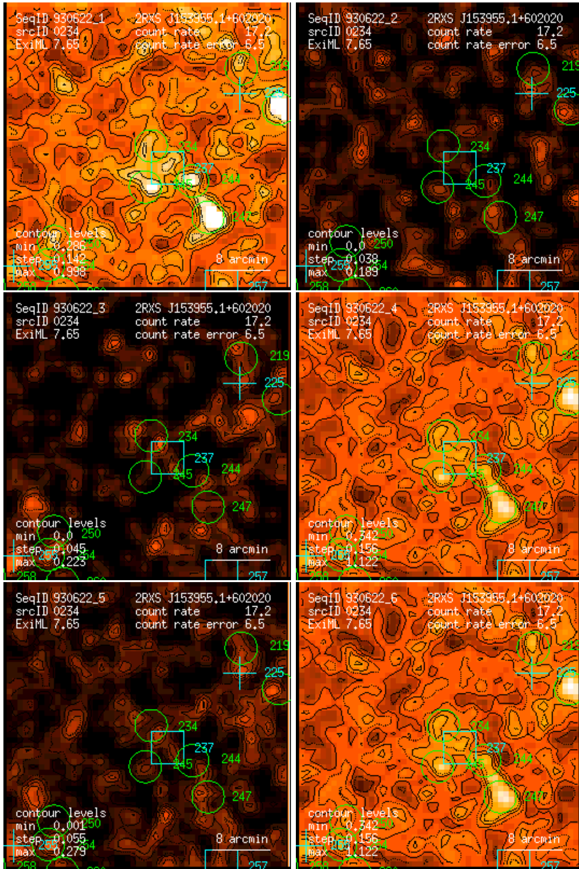
Figure 234: RASS 930622: detection 0234: band rate images, Gaussian filter: (1) PSPC channels 11 – 41, (2) 52 – 90, (3) 91 – 201, (4) 11 – 235, (5) 52 – 201, (6) 11 – 201. Broad band rates in counts/ks. Band rate contour levels in counts/ks/arcmin 2 .
