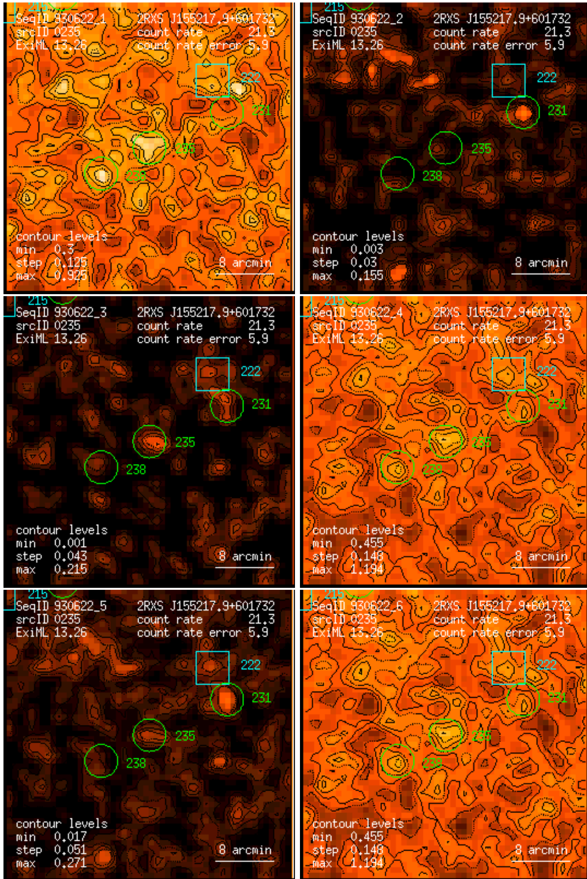
Figure 235: RASS 930622: detection 0235: band rate images, Gaussian filter: (1) PSPC channels 11 – 41, (2) 52 – 90, (3) 91 – 201, (4) 11 – 235, (5) 52 – 201, (6) 11 – 201. Broad band rates in counts/ks. Band rate contour levels in counts/ks/arcmin 2 .
