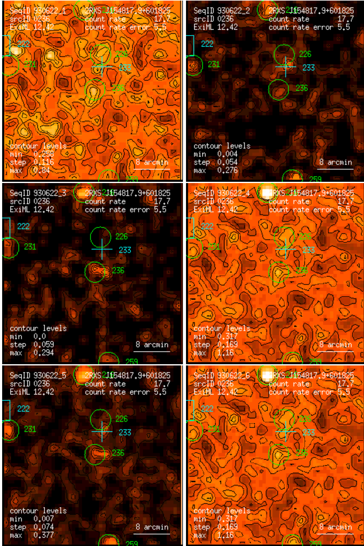
Figure 236: RASS 930622: detection 0236: band rate images, Gaussian filter: (1) PSPC channels 11 – 41, (2) 52 – 90, (3) 91 – 201, (4) 11 – 235, (5) 52 – 201, (6) 11 – 201. Broad band rates in counts/ks. Band rate contour levels in counts/ks/arcmin 2 .
