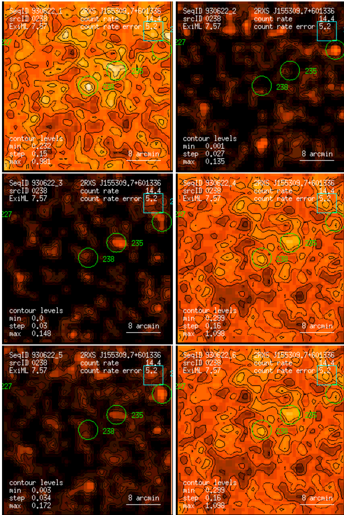
Figure 238: RASS 930622: detection 0238: band rate images, Gaussian filter: (1) PSPC channels 11 – 41, (2) 52 – 90, (3) 91 – 201, (4) 11 – 235, (5) 52 – 201, (6) 11 – 201. Broad band rates in counts/ks. Band rate contour levels in counts/ks/arcmin 2 .
