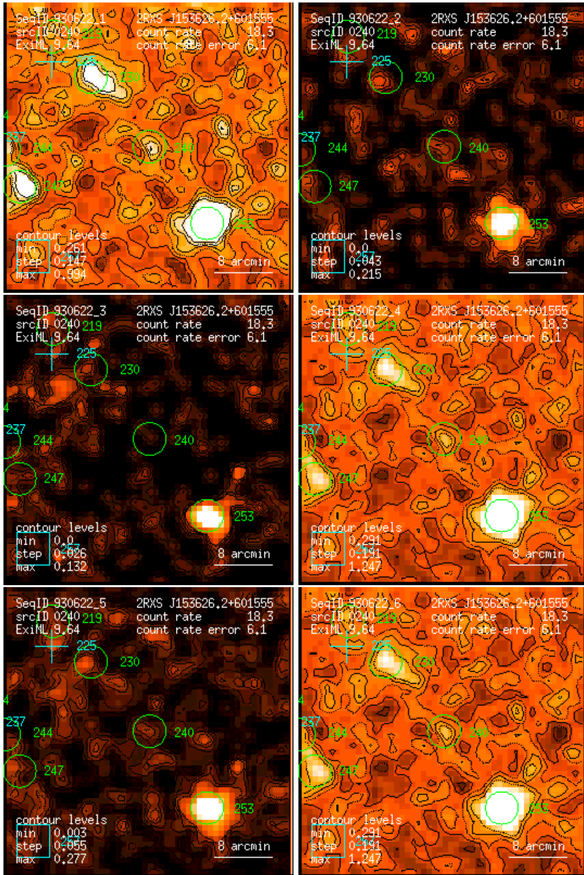
Figure 240: RASS 930622: detection 0240: band rate images, Gaussian filter: (1) PSPC channels 11 – 41, (2) 52 – 90, (3) 91 – 201, (4) 11 – 235, (5) 52 – 201, (6) 11 – 201. Broad band rates in counts/ks. Band rate contour levels in counts/ks/arcmin 2 .
