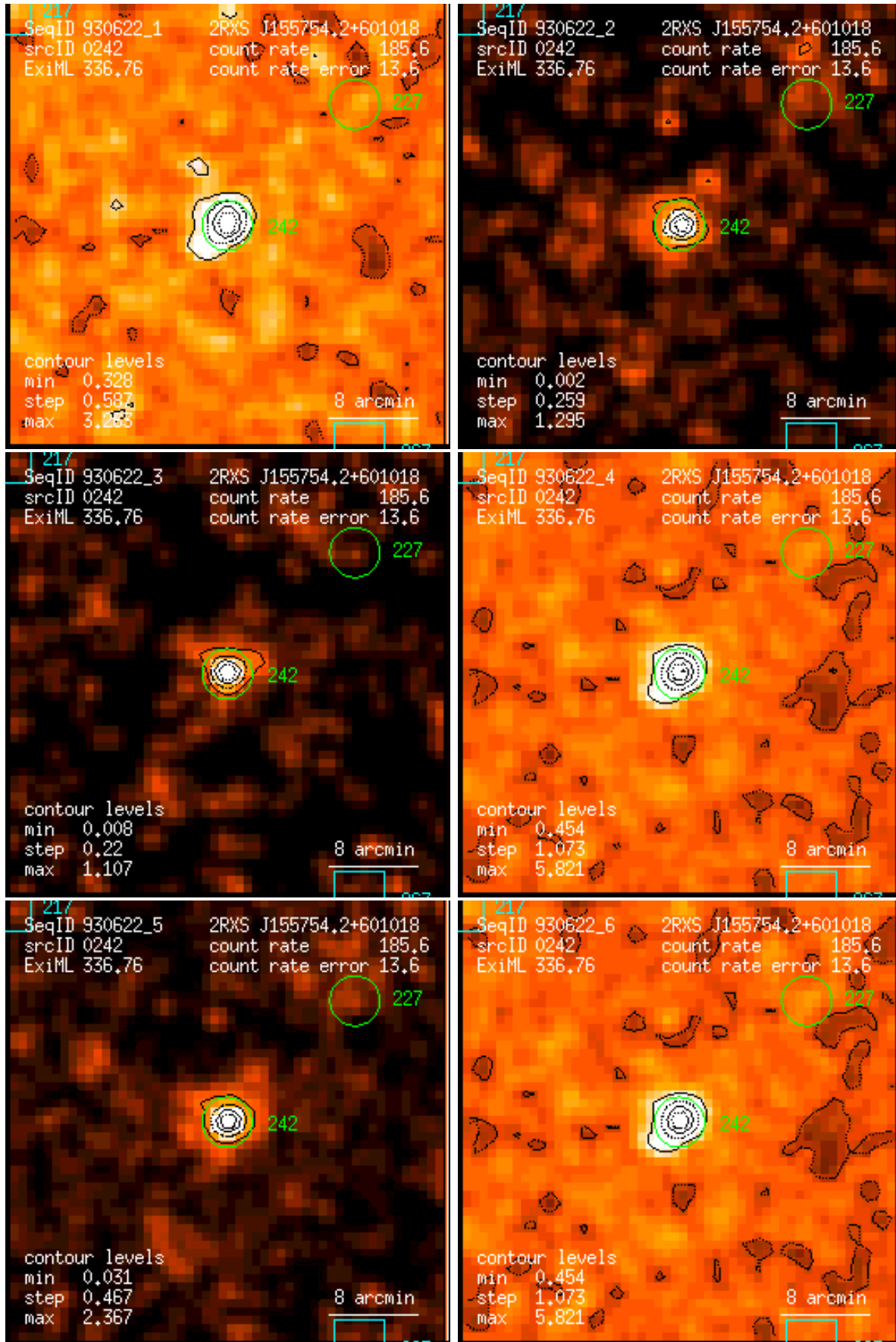
Figure 242: RASS 930622: detection 0242: band rate images, Gaussian filter: (1) PSPC channels 11 – 41, (2) 52 – 90, (3) 91 – 201, (4) 11 – 235, (5) 52 – 201, (6) 11 – 201. Broad band rates in counts/ks. Band rate contour levels in counts/ks/arcmin 2 .
