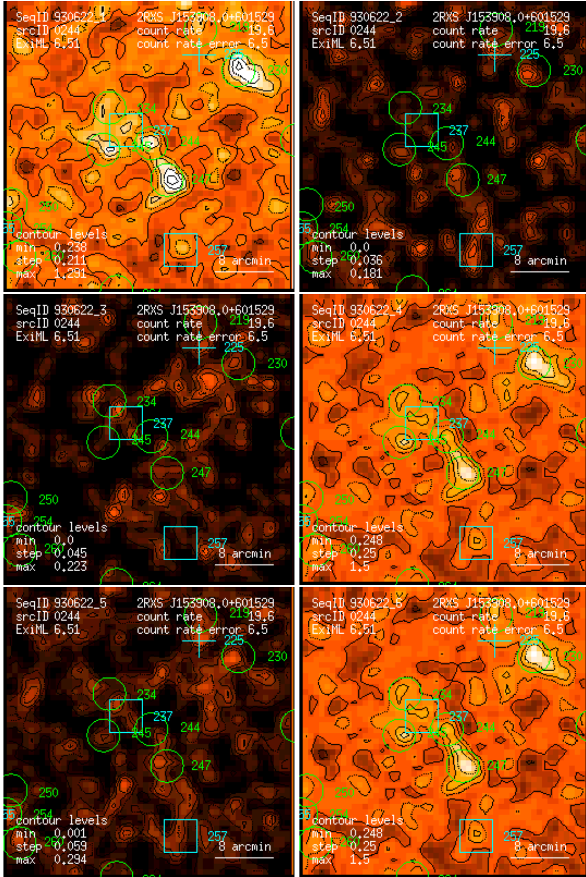
Figure 244: RASS 930622: detection 0244: band rate images, Gaussian filter: (1) PSPC channels 11 – 41, (2) 52 – 90, (3) 91 – 201, (4) 11 – 235, (5) 52 – 201, (6) 11 – 201. Broad band rates in counts/ks. Band rate contour levels in counts/ks/arcmin 2 .
