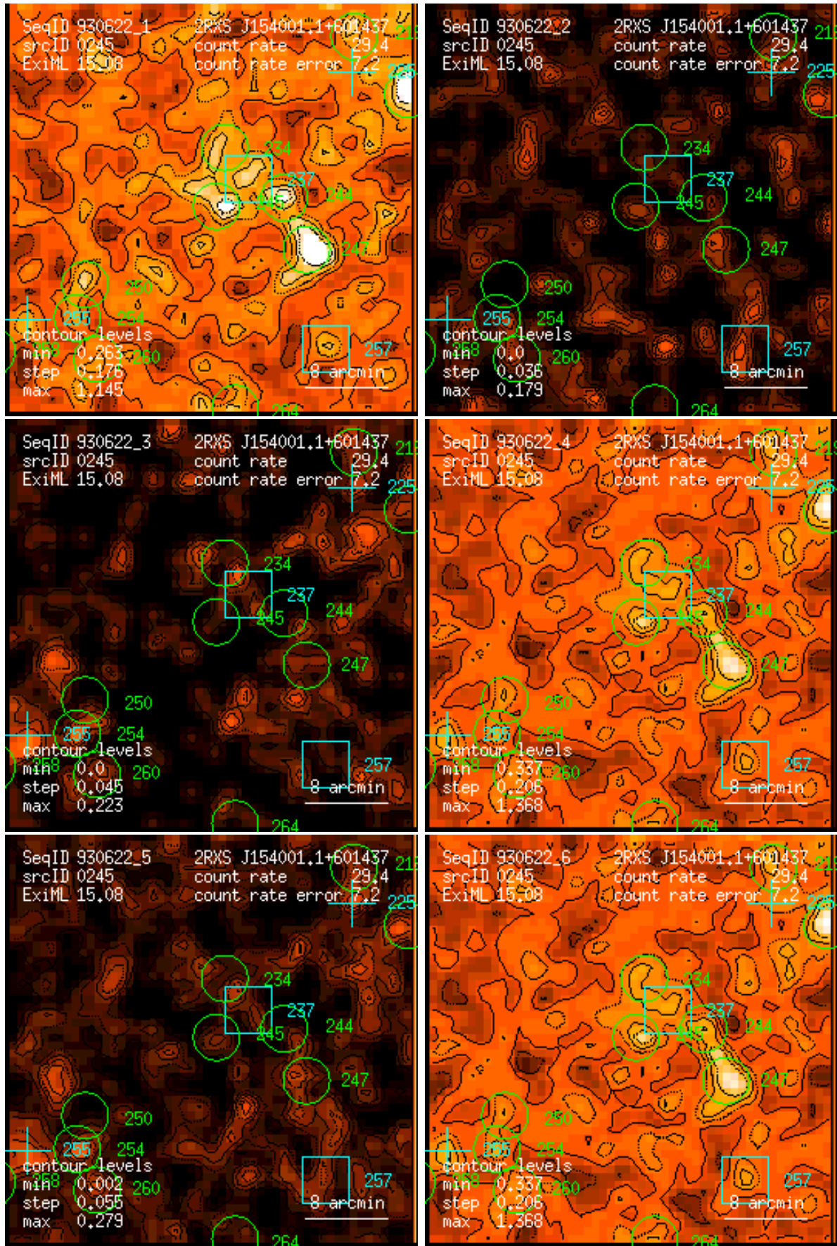
Figure 245: RASS 930622: detection 0245: band rate images, Gaussian filter: (1) PSPC channels 11 – 41, (2) 52 – 90, (3) 91 – 201, (4) 11 – 235, (5) 52 – 201, (6) 11 – 201. Broad band rates in counts/ks. Band rate contour levels in counts/ks/arcmin 2 .
