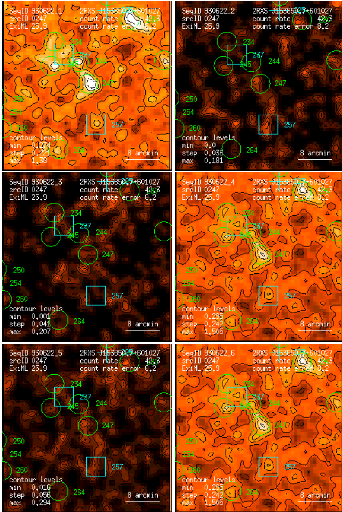
Figure 247: RASS 930622: detection 0247: band rate images, Gaussian filter: (1) PSPC channels 11 – 41, (2) 52 – 90, (3) 91 – 201, (4) 11 – 235, (5) 52 – 201, (6) 11 – 201. Broad band rates in counts/ks. Band rate contour levels in counts/ks/arcmin 2 .
