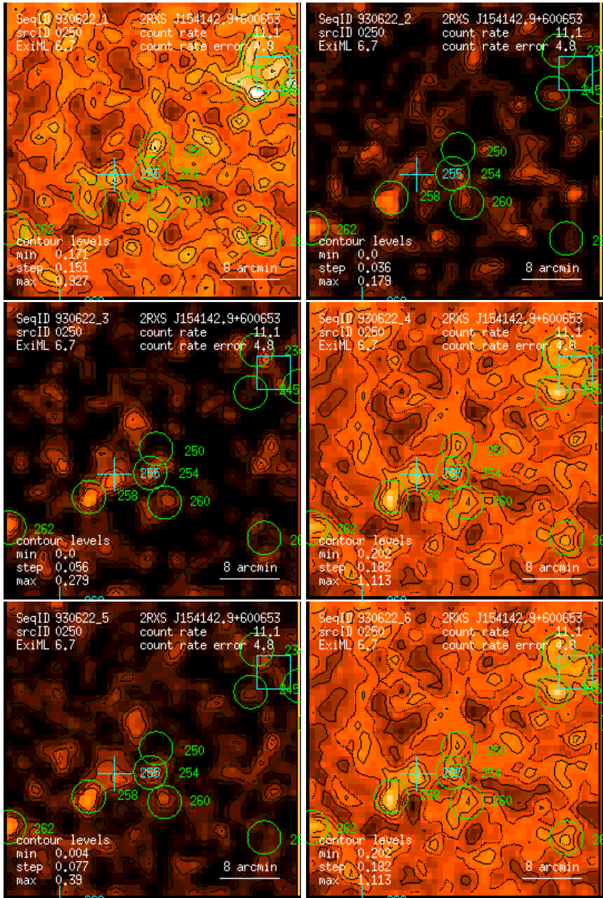
Figure 250: RASS 930622: detection 0250: band rate images, Gaussian filter: (1) PSPC channels 11 – 41, (2) 52 – 90, (3) 91 – 201, (4) 11 – 235, (5) 52 – 201, (6) 11 – 201. Broad band rates in counts/ks. Band rate contour levels in counts/ks/arcmin 2 .
