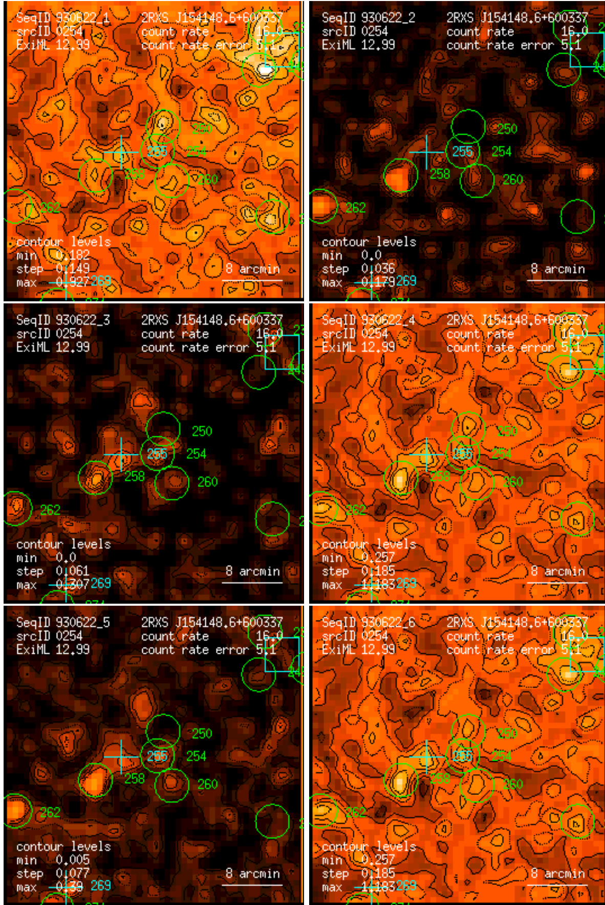
Figure 254: RASS 930622: detection 0254: band rate images, Gaussian filter: (1) PSPC channels 11 – 41, (2) 52 – 90, (3) 91 – 201, (4) 11 – 235, (5) 52 – 201, (6) 11 – 201. Broad band rates in counts/ks. Band rate contour levels in counts/ks/arcmin 2 .
