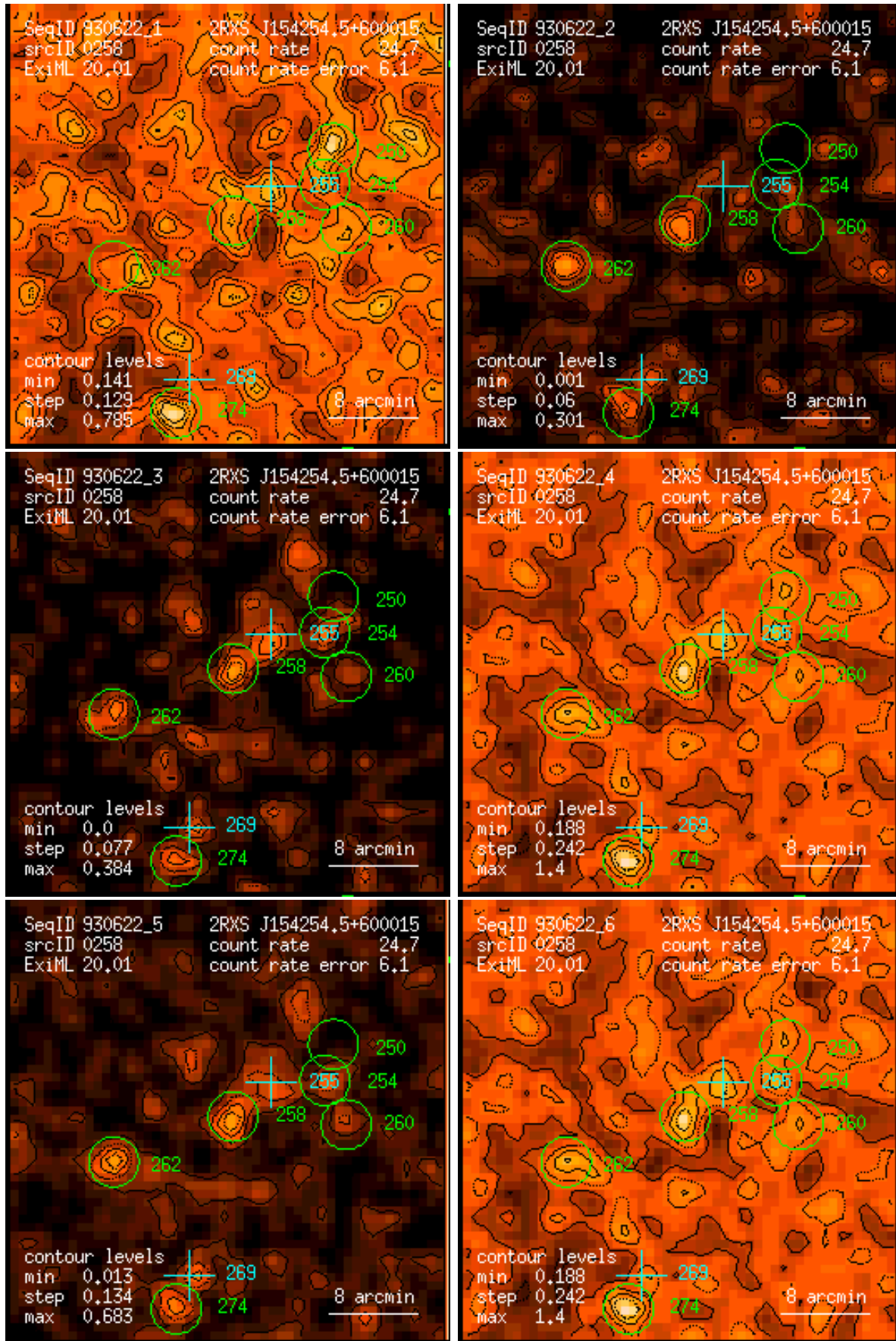
Figure 258: RASS 930622: detection 0258: band rate images, Gaussian filter: (1) PSPC channels 11 – 41, (2) 52 – 90, (3) 91 – 201, (4) 11 – 235, (5) 52 – 201, (6) 11 – 201. Broad band rates in counts/ks. Band rate contour levels in counts/ks/arcmin 2 .
