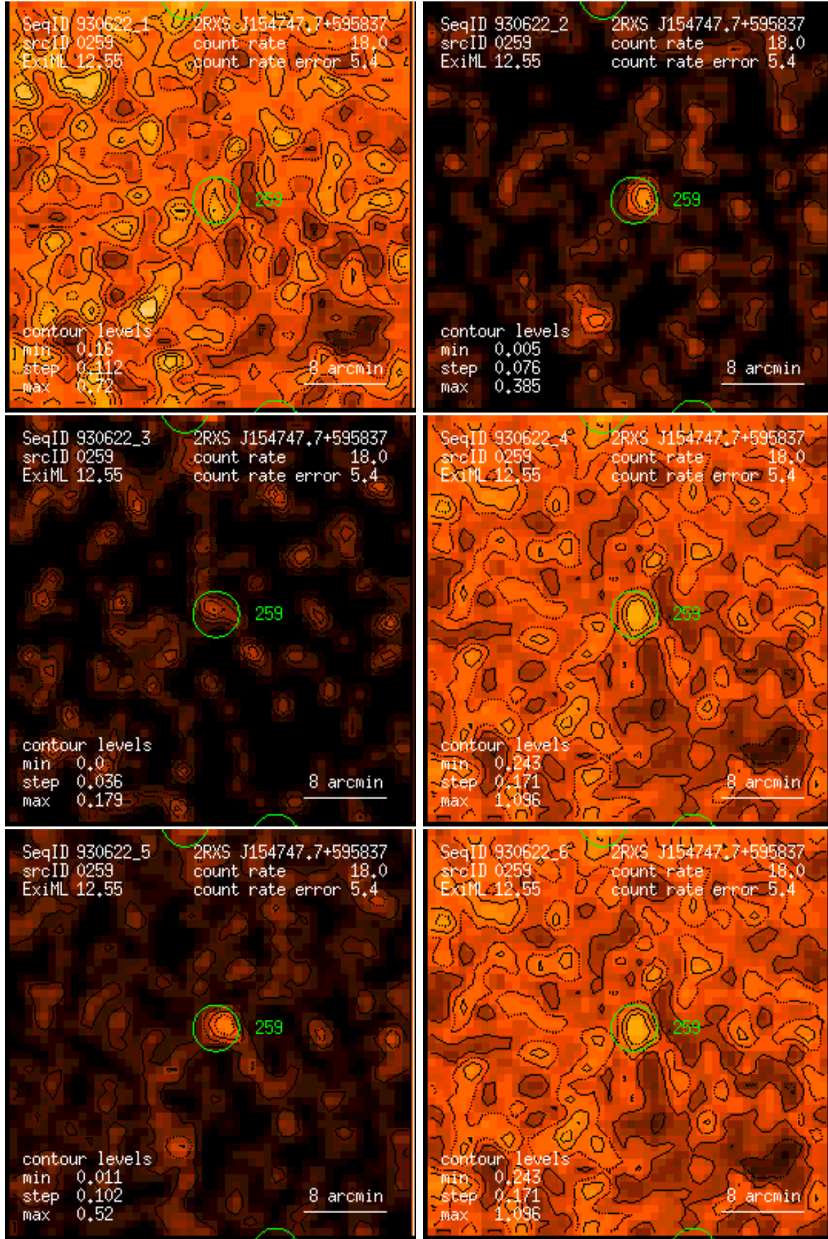
Figure 259: RASS 930622: detection 0259: band rate images, Gaussian filter: (1) PSPC channels 11 – 41, (2) 52 – 90, (3) 91 – 201, (4) 11 – 235, (5) 52 – 201, (6) 11 – 201. Broad band rates in counts/ks. Band rate contour levels in counts/ks/arcmin 2 .
