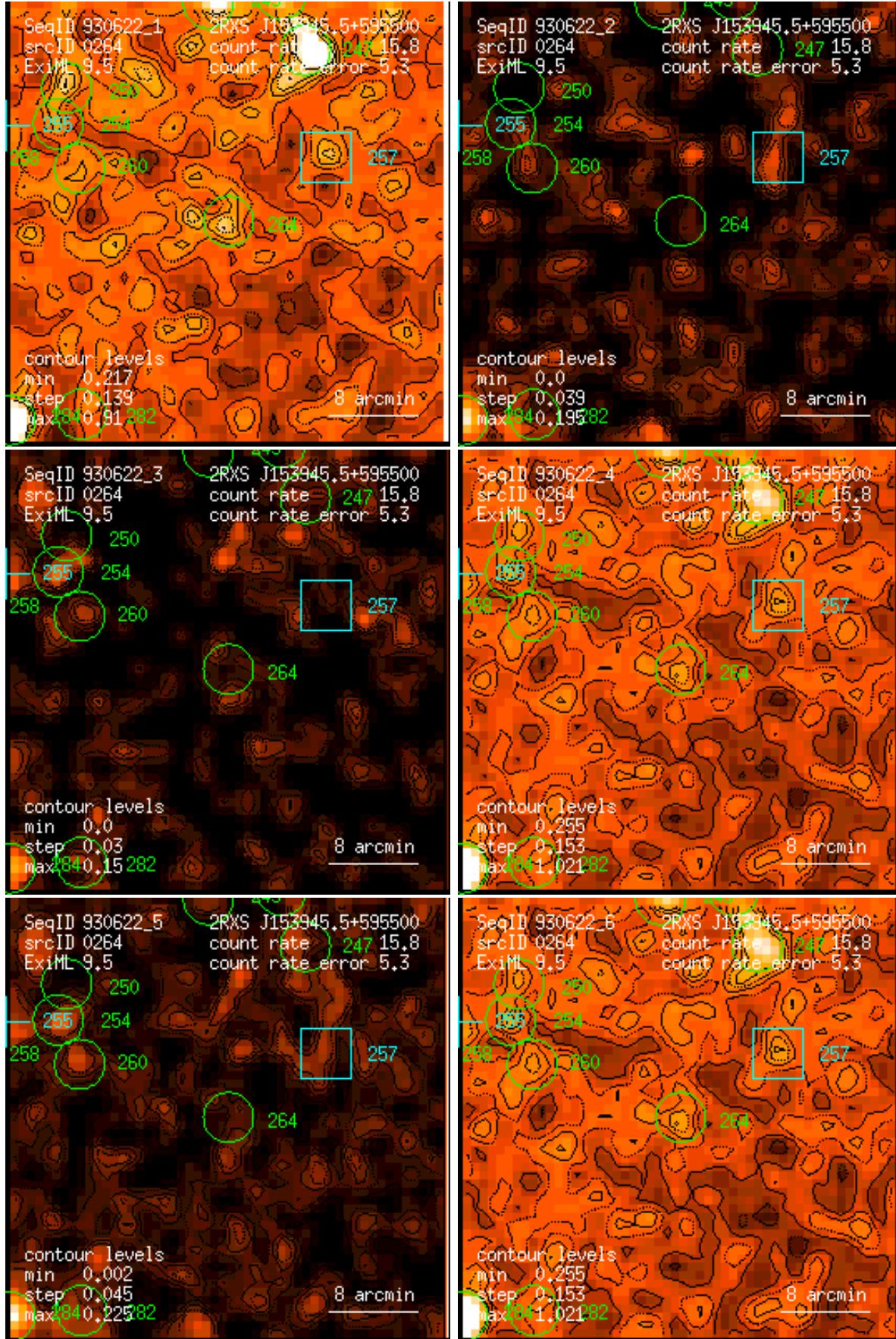
Figure 264: RASS 930622: detection 0264: band rate images, Gaussian filter: (1) PSPC channels 11 – 41, (2) 52 – 90, (3) 91 – 201, (4) 11 – 235, (5) 52 – 201, (6) 11 – 201. Broad band rates in counts/ks. Band rate contour levels in counts/ks/arcmin 2 .
