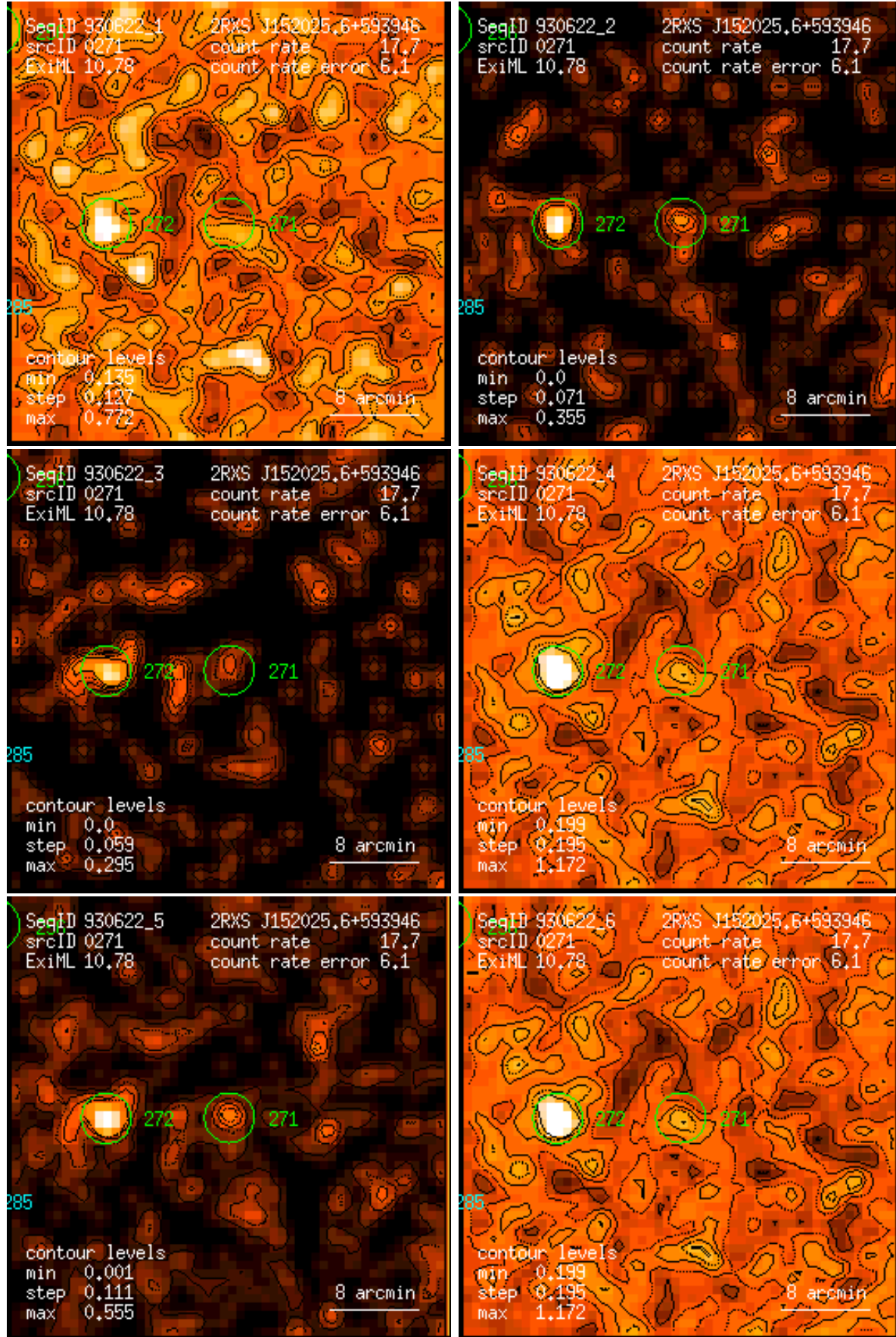
Figure 271: RASS 930622: detection 0271: band rate images, Gaussian filter: (1) PSPC channels 11 – 41, (2) 52 – 90, (3) 91 – 201, (4) 11 – 235, (5) 52 – 201, (6) 11 – 201. Broad band rates in counts/ks. Band rate contour levels in counts/ks/arcmin 2 .
