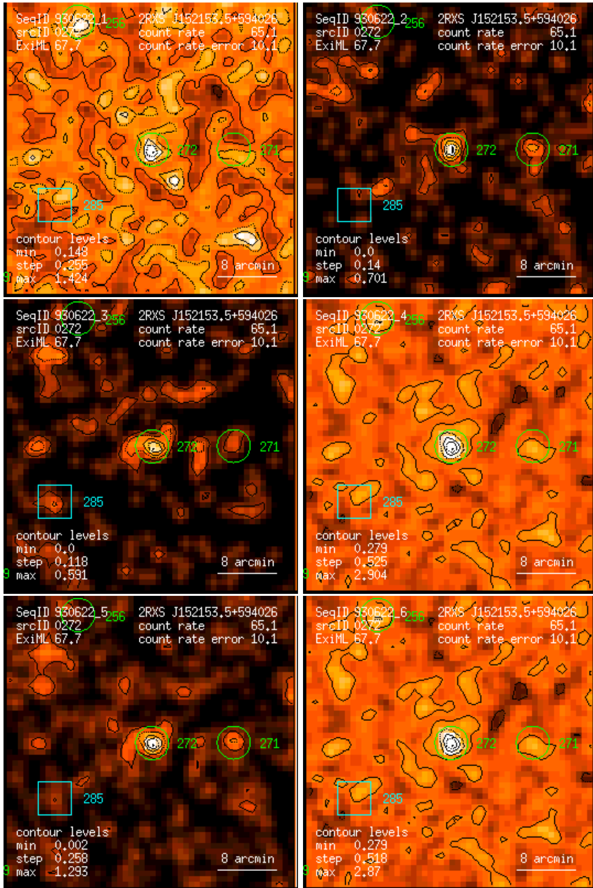
Figure 272: RASS 930622: detection 0272: band rate images, Gaussian filter: (1) PSPC channels 11 – 41, (2) 52 – 90, (3) 91 – 201, (4) 11 – 235, (5) 52 – 201, (6) 11 – 201. Broad band rates in counts/ks. Band rate contour levels in counts/ks/arcmin 2 .
