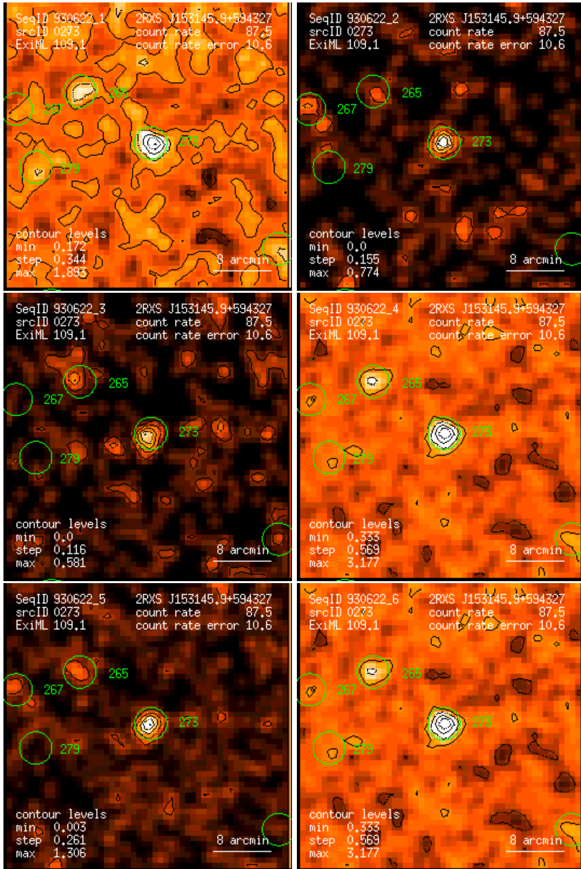
Figure 273: RASS 930622: detection 0273: band rate images, Gaussian filter: (1) PSPC channels 11 – 41, (2) 52 – 90, (3) 91 – 201, (4) 11 – 235, (5) 52 – 201, (6) 11 – 201. Broad band rates in counts/ks. Band rate contour levels in counts/ks/arcmin 2 .
