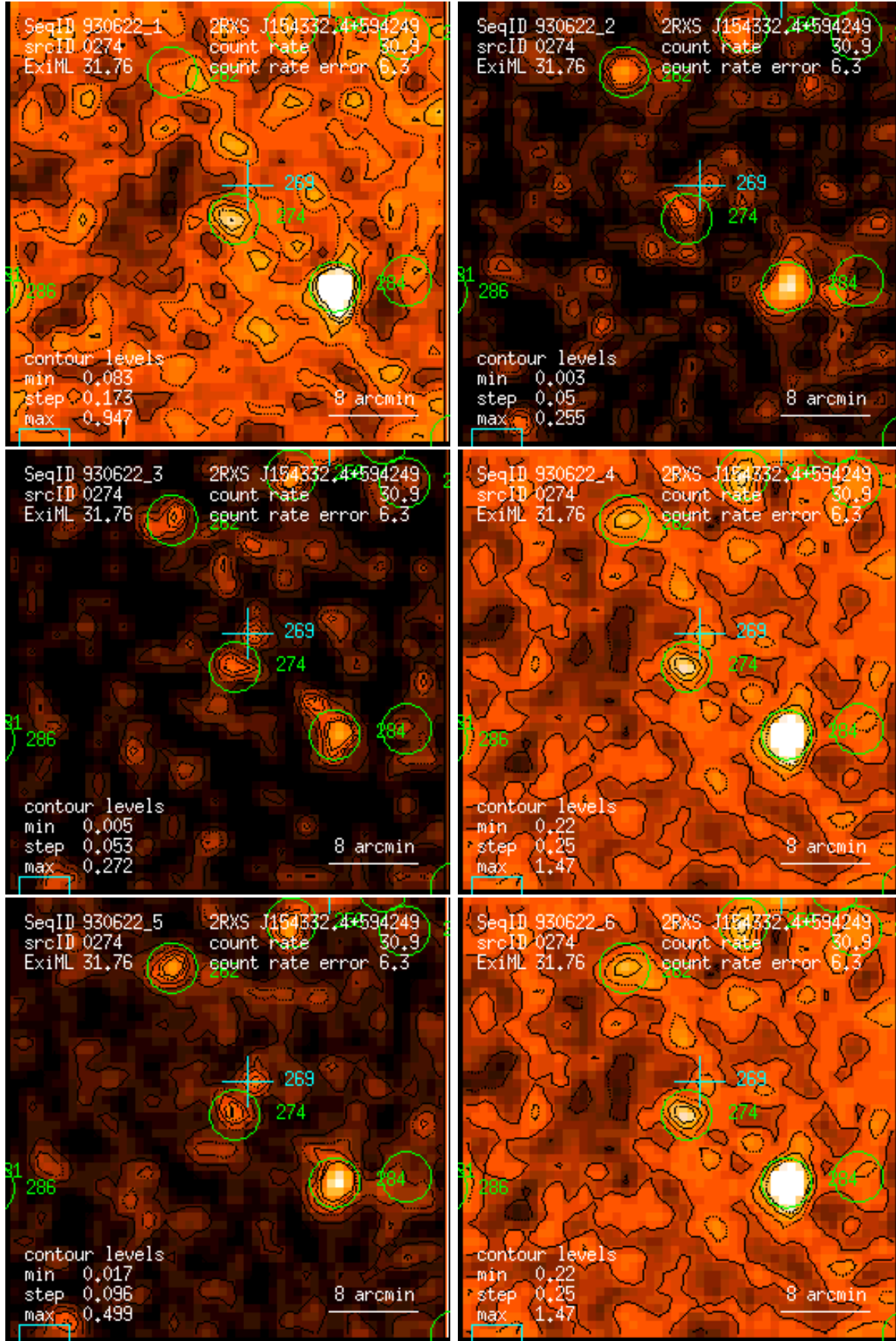
Figure 274: RASS 930622: detection 0274: band rate images, Gaussian filter: (1) PSPC channels 11 – 41, (2) 52 – 90, (3) 91 – 201, (4) 11 – 235, (5) 52 – 201, (6) 11 – 201. Broad band rates in counts/ks. Band rate contour levels in counts/ks/arcmin 2 .
