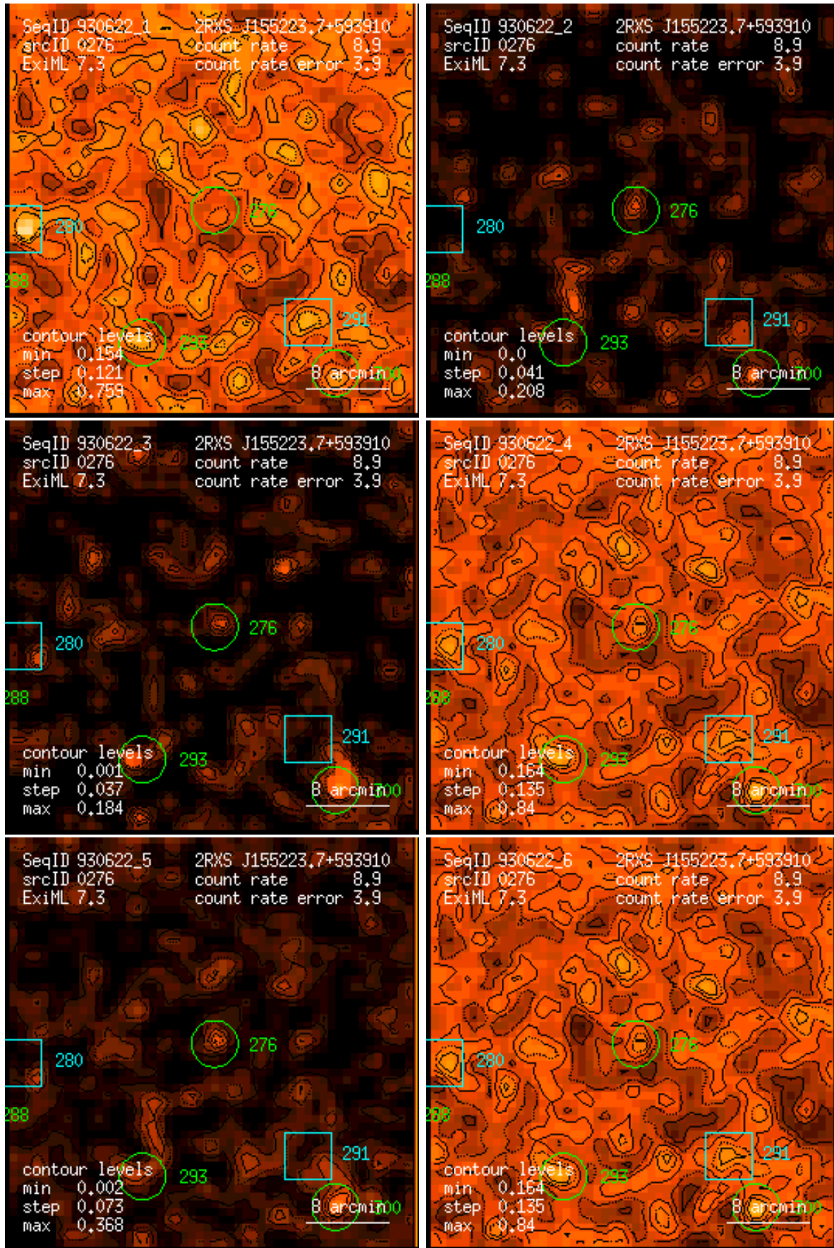
Figure 276: RASS 930622: detection 0276: band rate images, Gaussian filter: (1) PSPC channels 11 – 41, (2) 52 – 90, (3) 91 – 201, (4) 11 – 235, (5) 52 – 201, (6) 11 – 201. Broad band rates in counts/ks. Band rate contour levels in counts/ks/arcmin 2 .
