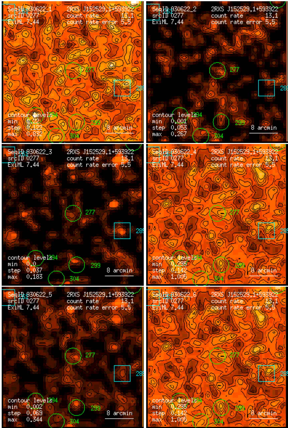
Figure 277: RASS 930622: detection 0277: band rate images, Gaussian filter: (1) PSPC channels 11 – 41, (2) 52 – 90, (3) 91 – 201, (4) 11 – 235, (5) 52 – 201, (6) 11 – 201. Broad band rates in counts/ks. Band rate contour levels in counts/ks/arcmin 2 .
