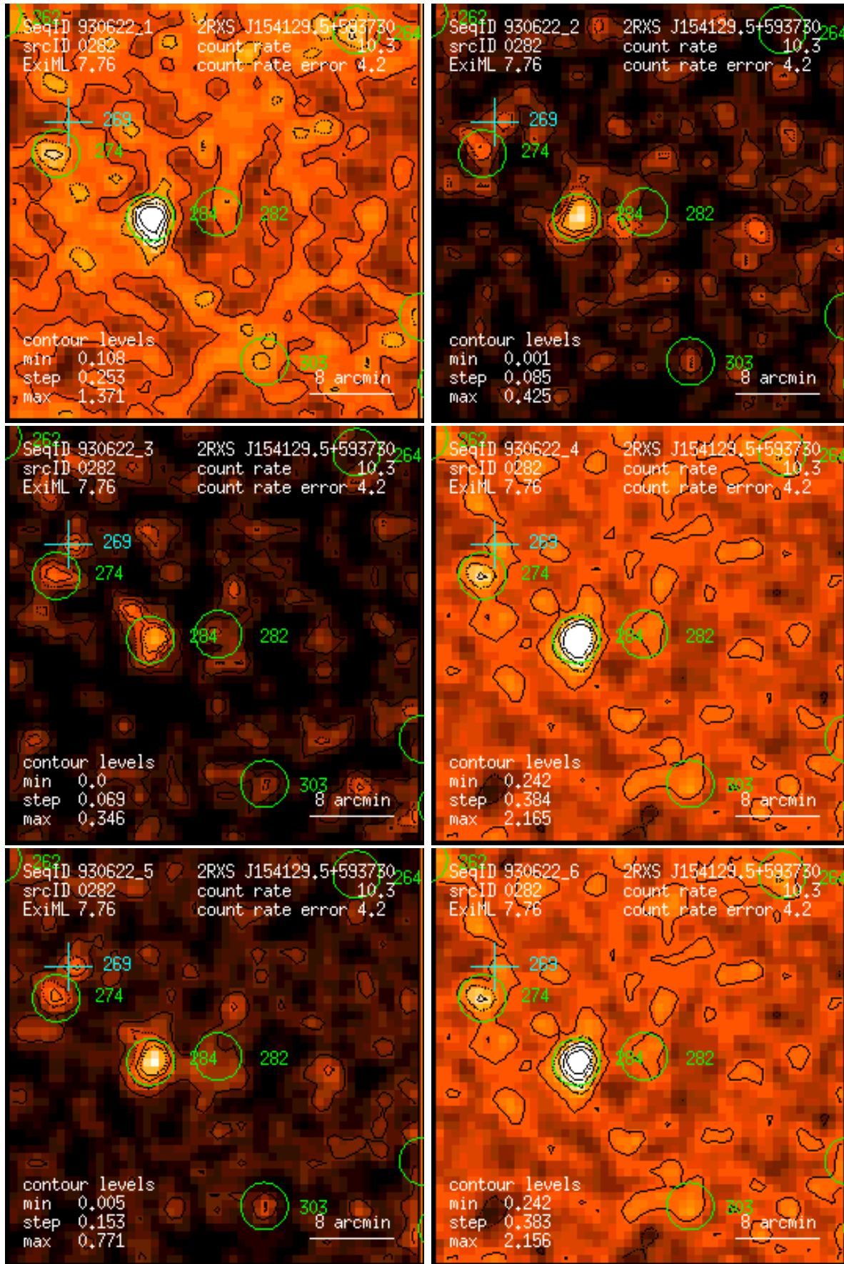
Figure 282: RASS 930622: detection 0282: band rate images, Gaussian filter: (1) PSPC channels 11 – 41, (2) 52 – 90, (3) 91 – 201, (4) 11 – 235, (5) 52 – 201, (6) 11 – 201. Broad band rates in counts/ks. Band rate contour levels in counts/ks/arcmin 2 .
