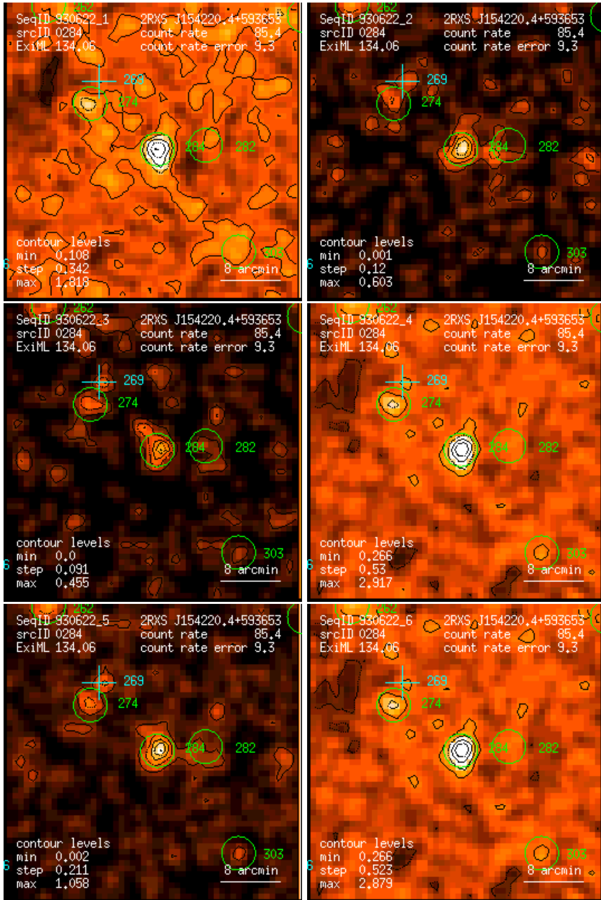
Figure 284: RASS 930622: detection 0284: band rate images, Gaussian filter: (1) PSPC channels 11 – 41, (2) 52 – 90, (3) 91 – 201, (4) 11 – 235, (5) 52 – 201, (6) 11 – 201. Broad band rates in counts/ks. Band rate contour levels in counts/ks/arcmin 2 .
