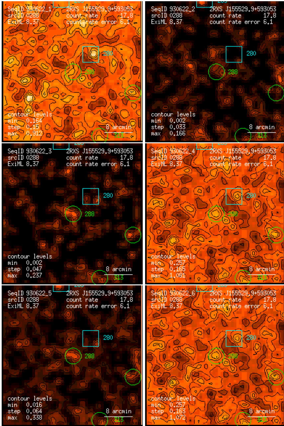
Figure 288: RASS 930622: detection 0288: band rate images, Gaussian filter: (1) PSPC channels 11 – 41, (2) 52 – 90, (3) 91 – 201, (4) 11 – 235, (5) 52 – 201, (6) 11 – 201. Broad band rates in counts/ks. Band rate contour levels in counts/ks/arcmin 2 .
