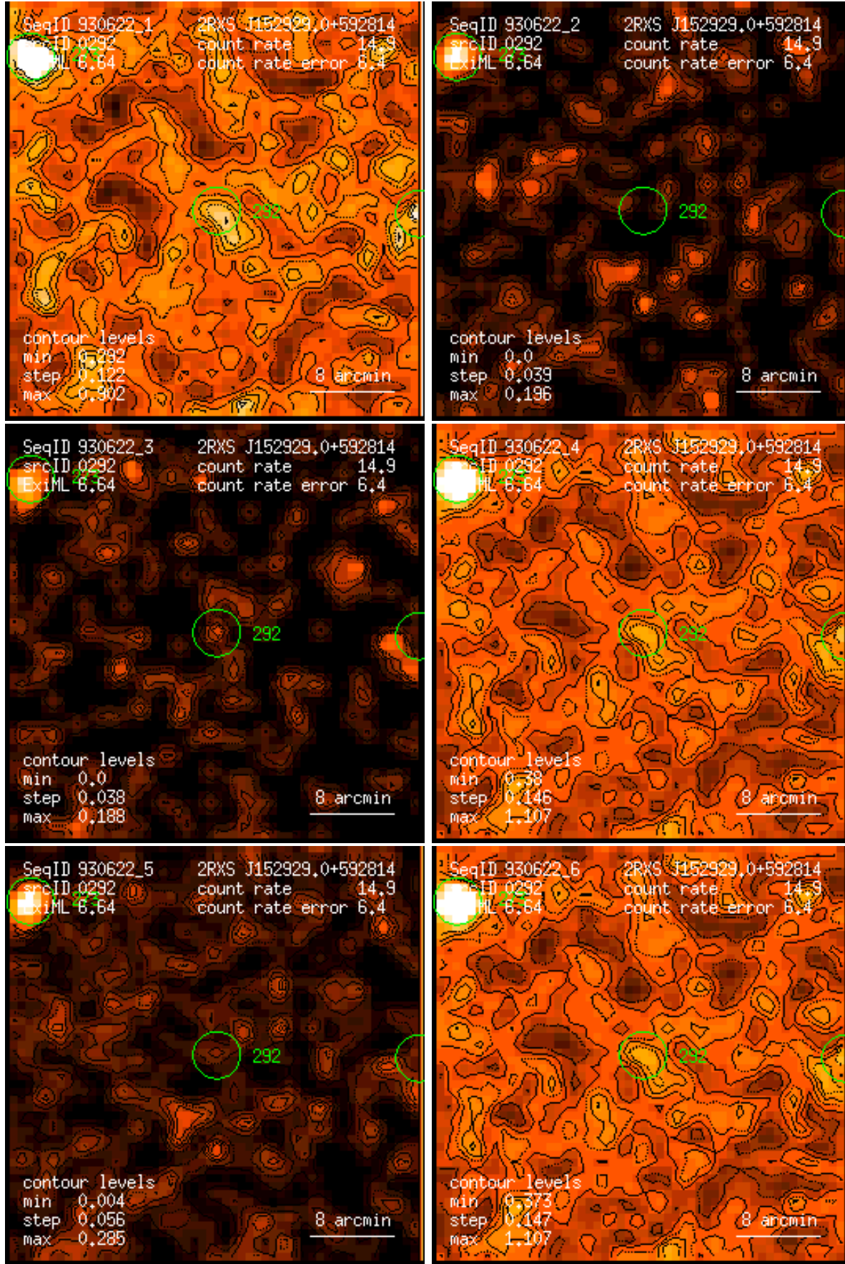
Figure 292: RASS 930622: detection 0292: band rate images, Gaussian filter: (1) PSPC channels 11 – 41, (2) 52 – 90, (3) 91 – 201, (4) 11 – 235, (5) 52 – 201, (6) 11 – 201. Broad band rates in counts/ks. Band rate contour levels in counts/ks/arcmin 2 .
