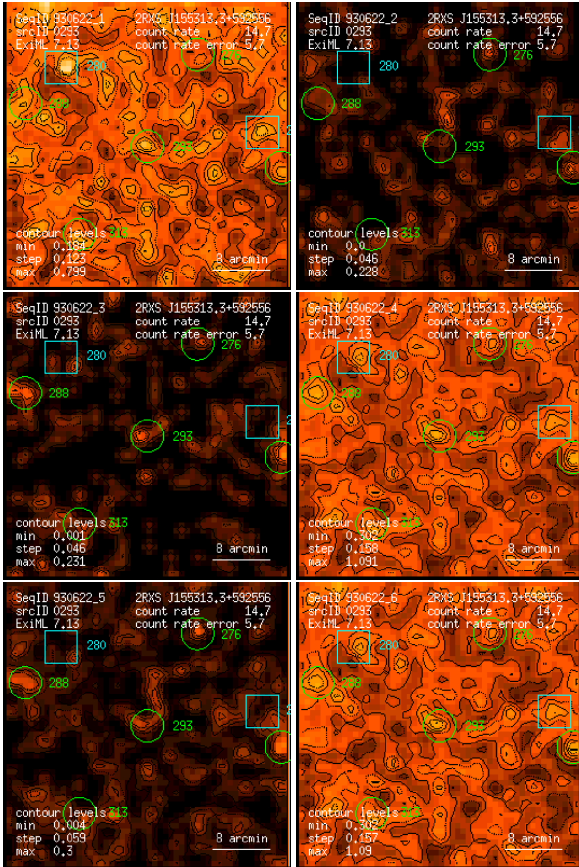
Figure 293: RASS 930622: detection 0293: band rate images, Gaussian filter: (1) PSPC channels 11 – 41, (2) 52 – 90, (3) 91 – 201, (4) 11 – 235, (5) 52 – 201, (6) 11 – 201. Broad band rates in counts/ks. Band rate contour levels in counts/ks/arcmin 2 .
