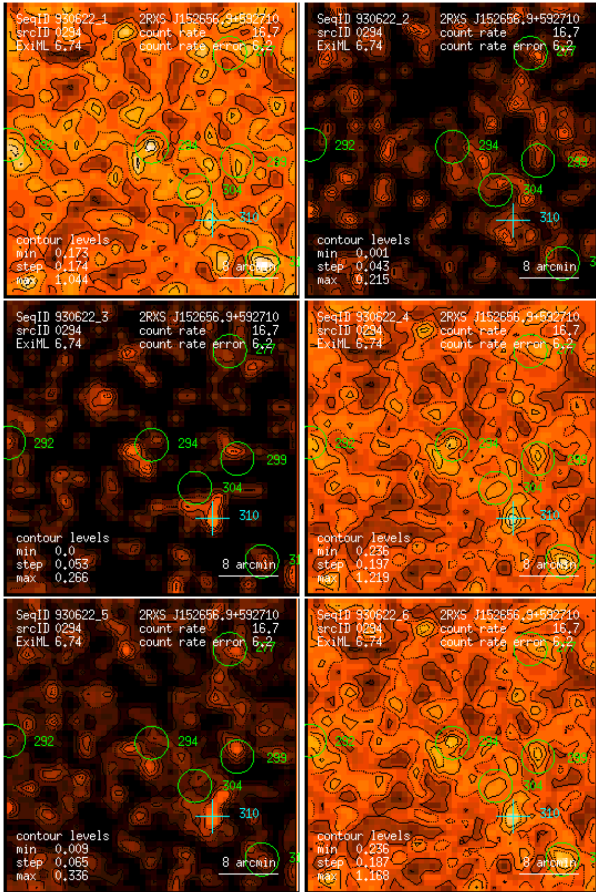
Figure 294: RASS 930622: detection 0294: band rate images, Gaussian filter: (1) PSPC channels 11 – 41, (2) 52 – 90, (3) 91 – 201, (4) 11 – 235, (5) 52 – 201, (6) 11 – 201. Broad band rates in counts/ks. Band rate contour levels in counts/ks/arcmin 2 .
