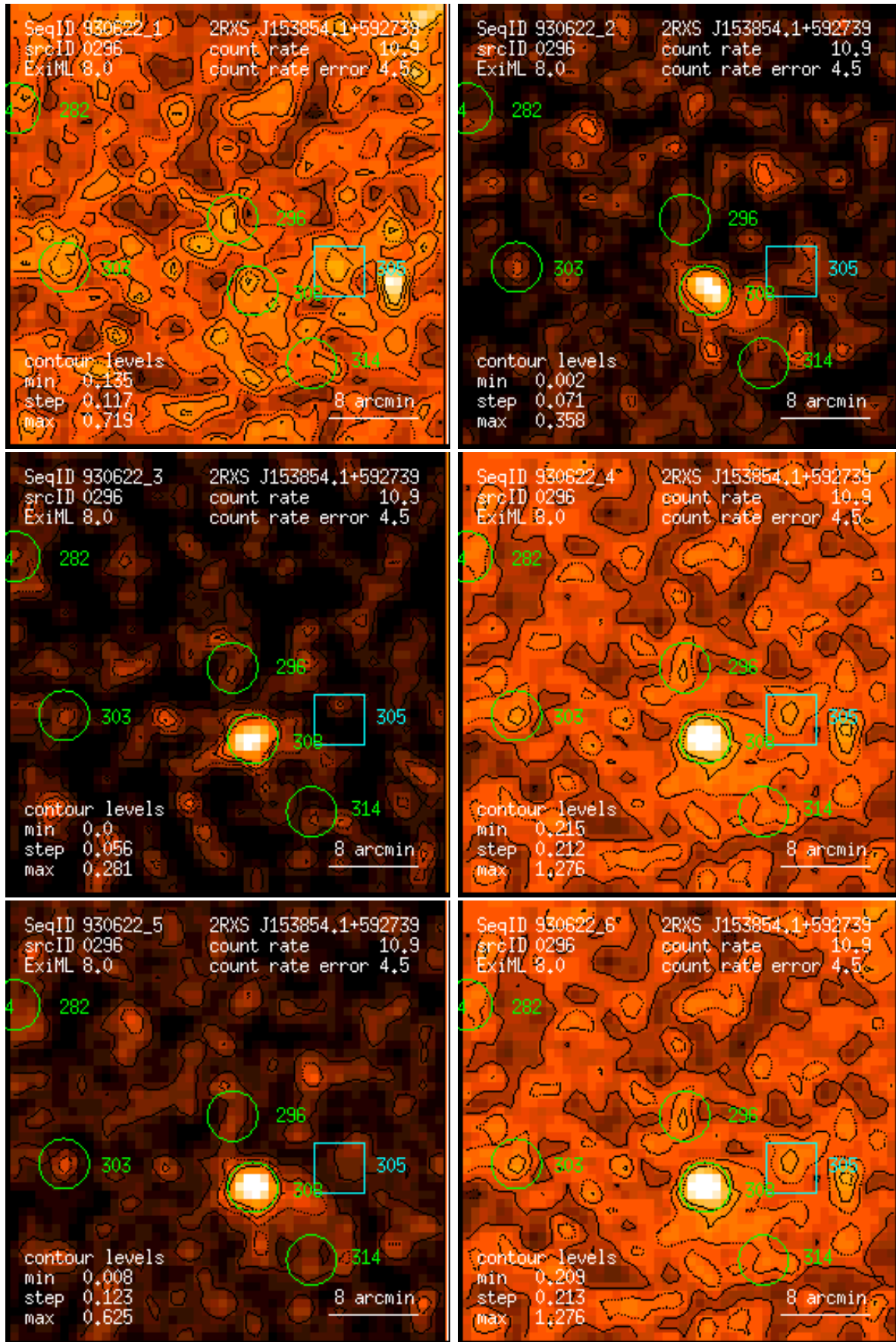
Figure 296: RASS 930622: detection 0296: band rate images, Gaussian filter: (1) PSPC channels 11 – 41, (2) 52 – 90, (3) 91 – 201, (4) 11 – 235, (5) 52 – 201, (6) 11 – 201. Broad band rates in counts/ks. Band rate contour levels in counts/ks/arcmin 2 .
