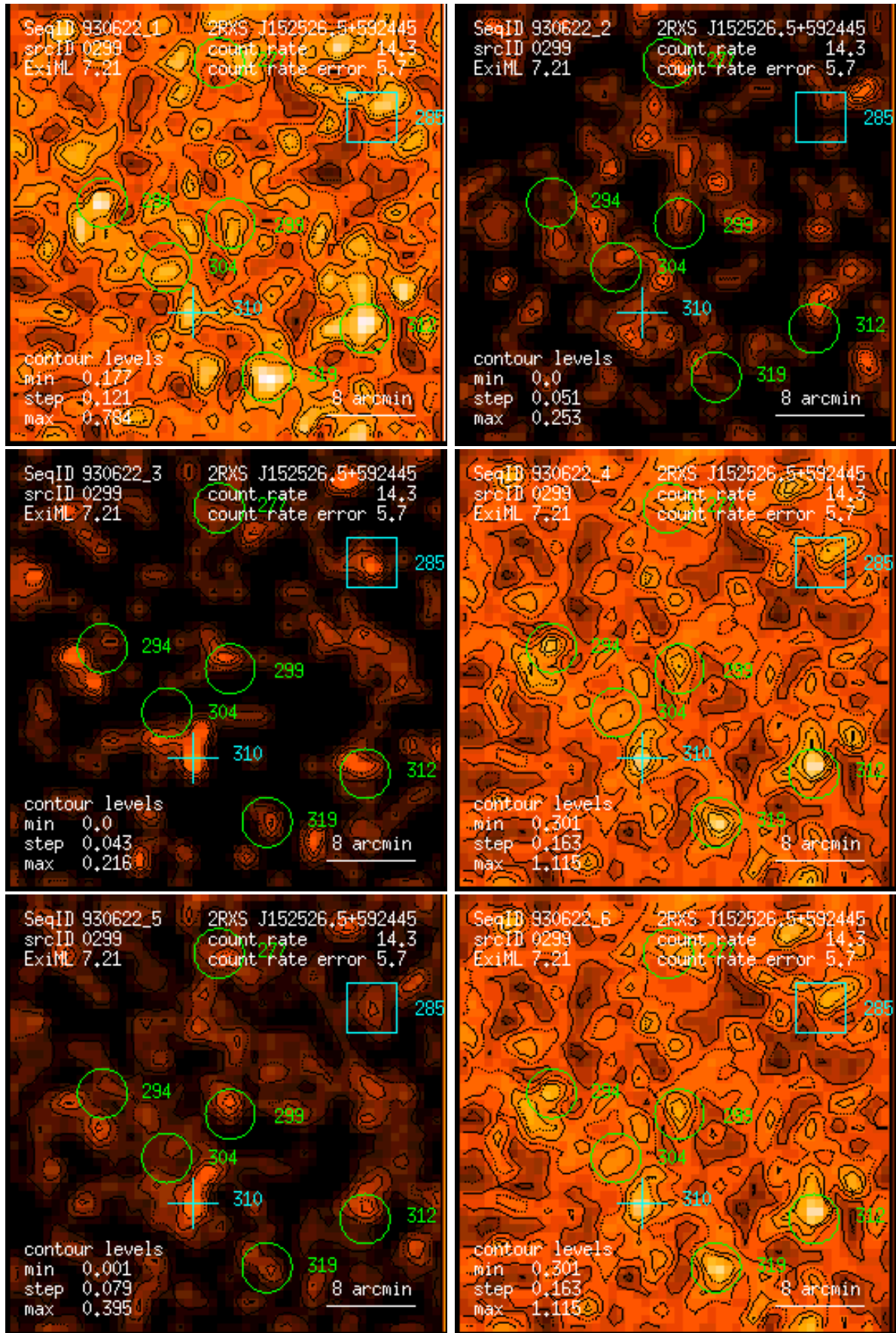
Figure 299: RASS 930622: detection 0299: band rate images, Gaussian filter: (1) PSPC channels 11 – 41, (2) 52 – 90, (3) 91 – 201, (4) 11 – 235, (5) 52 – 201, (6) 11 – 201. Broad band rates in counts/ks. Band rate contour levels in counts/ks/arcmin 2 .
