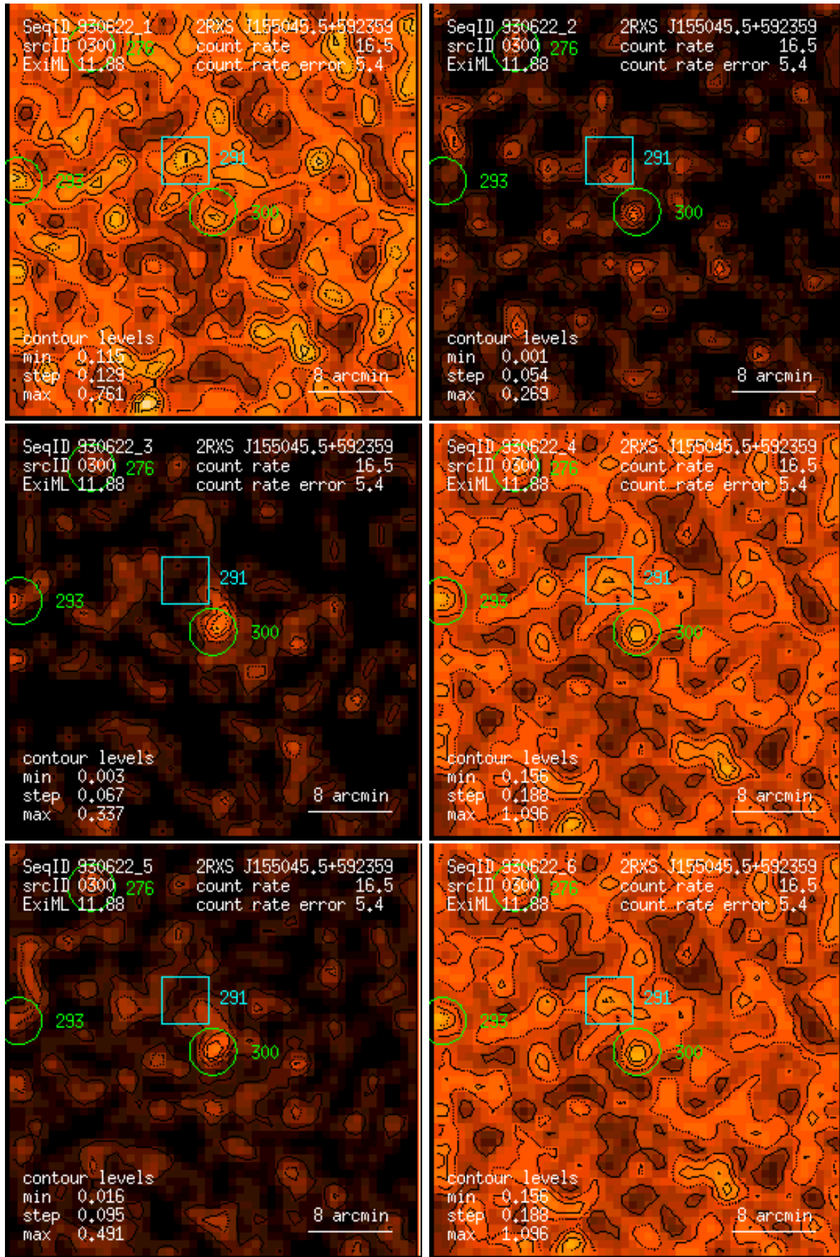
Figure 300: RASS 930622: detection 0300: band rate images, Gaussian filter: (1) PSPC channels 11 – 41, (2) 52 – 90, (3) 91 – 201, (4) 11 – 235, (5) 52 – 201, (6) 11 – 201. Broad band rates in counts/ks. Band rate contour levels in counts/ks/arcmin 2 .
