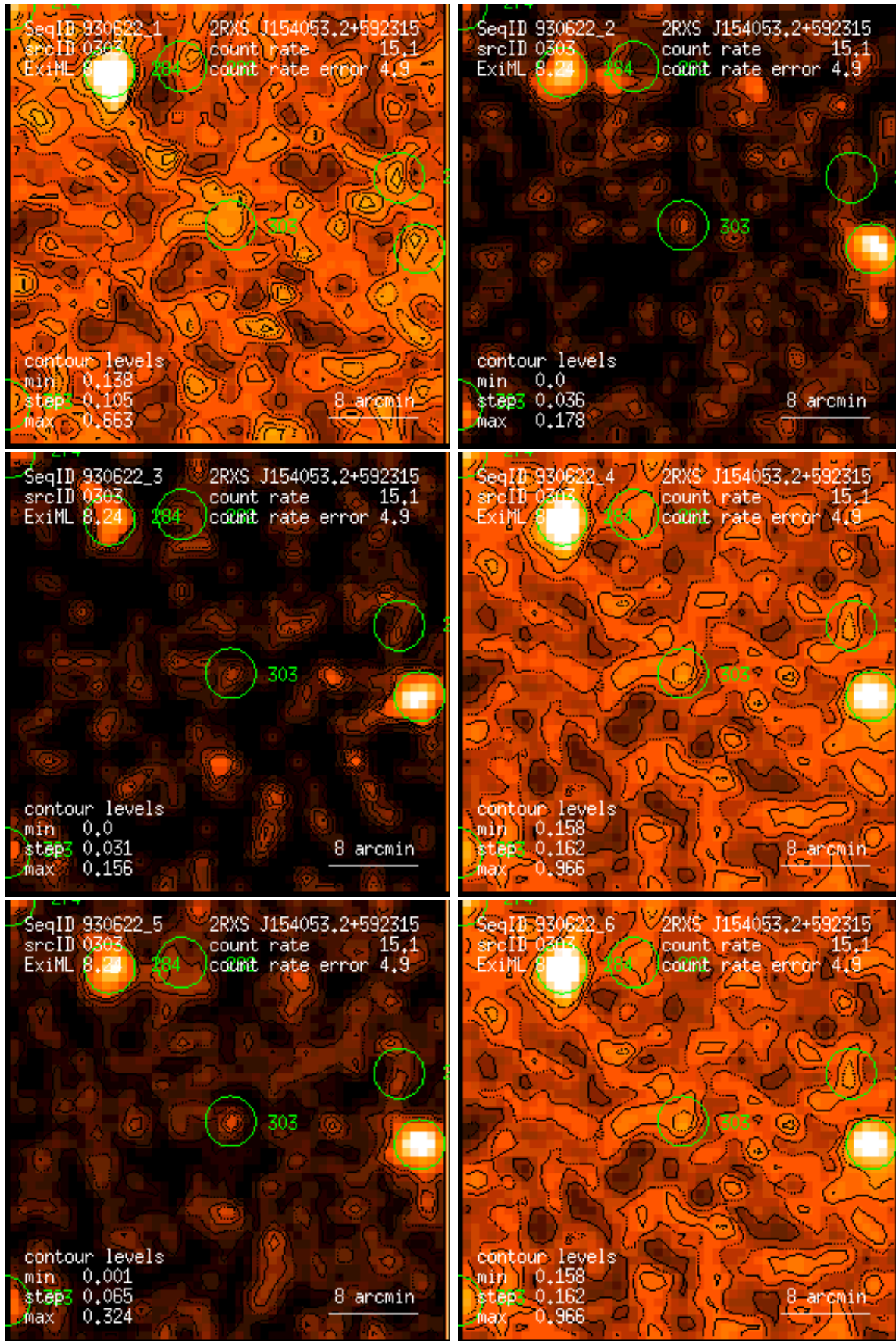
Figure 303: RASS 930622: detection 0303: band rate images, Gaussian filter: (1) PSPC channels 11 – 41, (2) 52 – 90, (3) 91 – 201, (4) 11 – 235, (5) 52 – 201, (6) 11 – 201. Broad band rates in counts/ks. Band rate contour levels in counts/ks/arcmin 2 .
