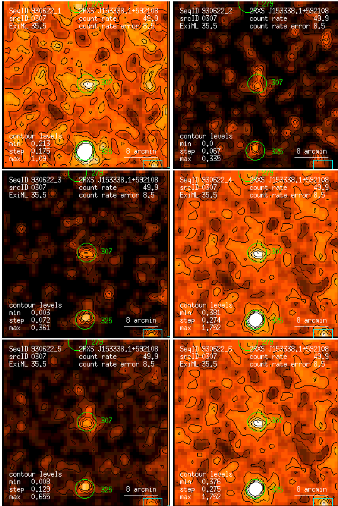
Figure 307: RASS 930622: detection 0307: band rate images, Gaussian filter: (1) PSPC channels 11 – 41, (2) 52 – 90, (3) 91 – 201, (4) 11 – 235, (5) 52 – 201, (6) 11 – 201. Broad band rates in counts/ks. Band rate contour levels in counts/ks/arcmin 2 .
