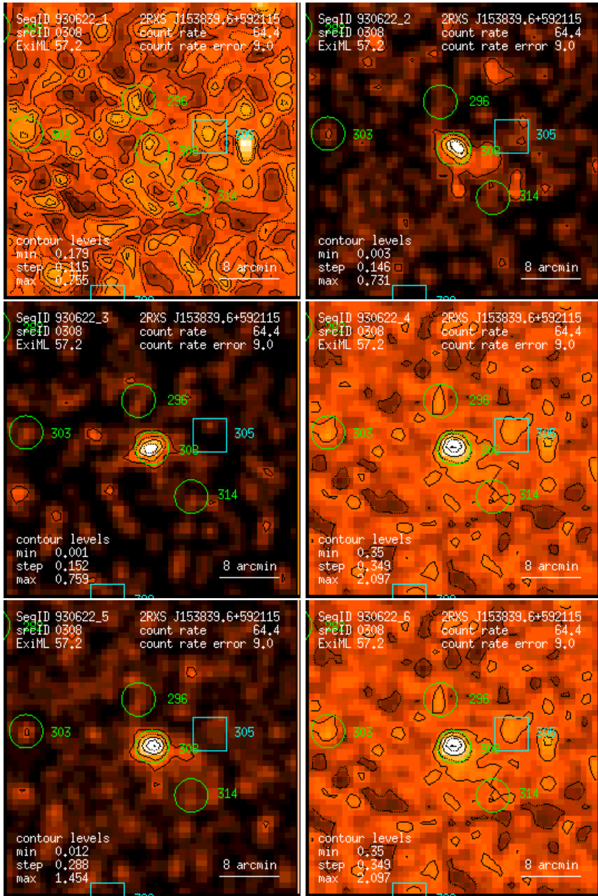
Figure 308: RASS 930622: detection 0308: band rate images, Gaussian filter: (1) PSPC channels 11 – 41, (2) 52 – 90, (3) 91 – 201, (4) 11 – 235, (5) 52 – 201, (6) 11 – 201. Broad band rates in counts/ks. Band rate contour levels in counts/ks/arcmin 2 .
