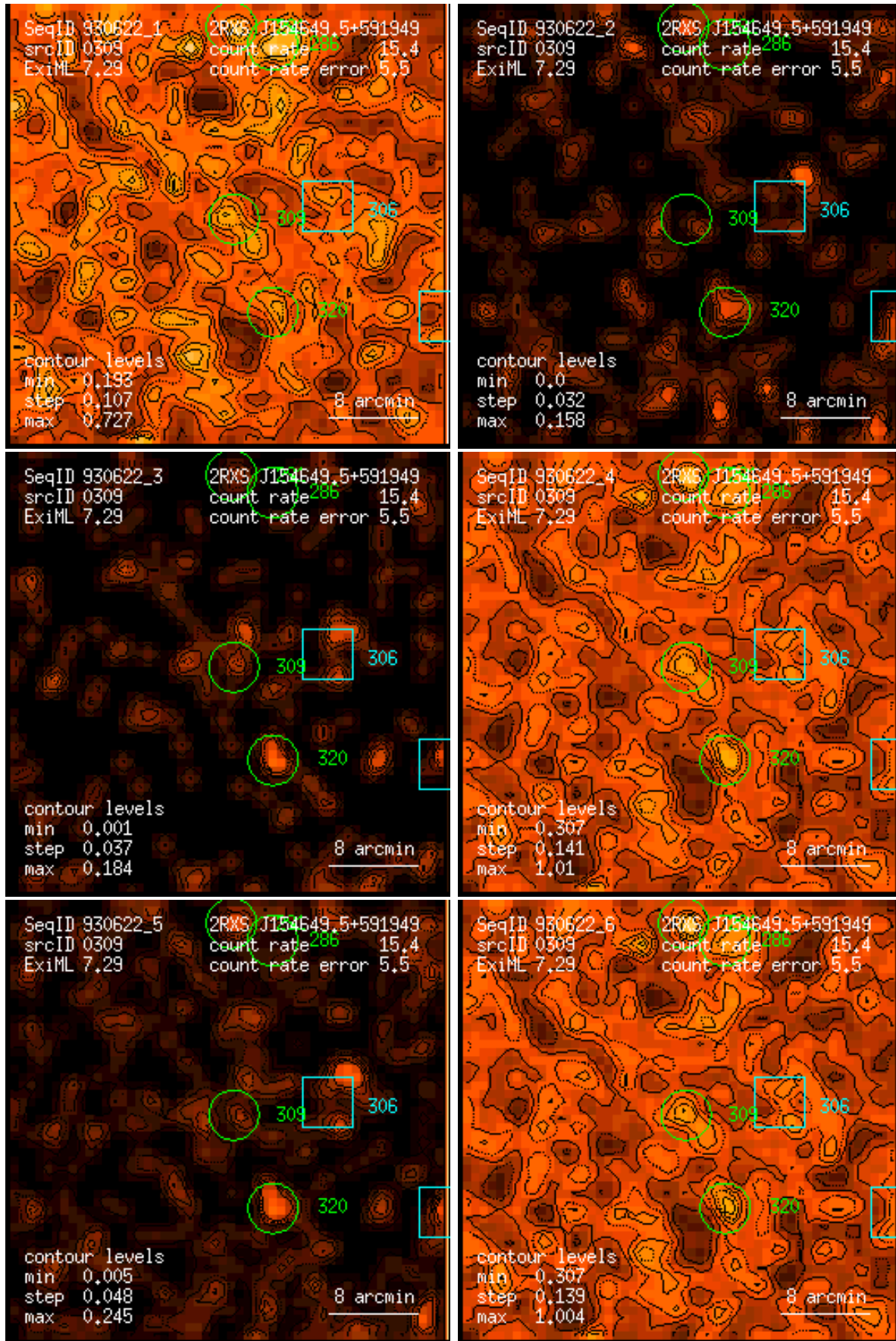
Figure 309: RASS 930622: detection 0309: band rate images, Gaussian filter: (1) PSPC channels 11 – 41, (2) 52 – 90, (3) 91 – 201, (4) 11 – 235, (5) 52 – 201, (6) 11 – 201. Broad band rates in counts/ks. Band rate contour levels in counts/ks/arcmin 2 .
