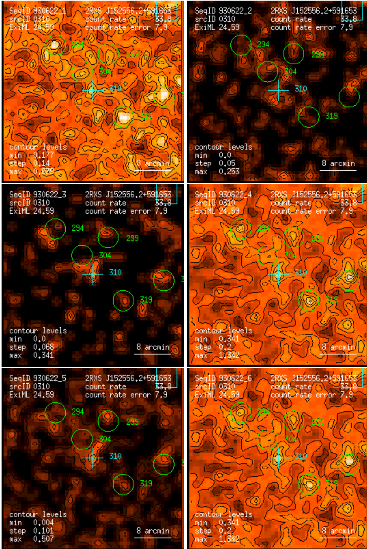
Figure 310: RASS 930622: detection 0310: band rate images, Gaussian filter: (1) PSPC channels 11 – 41, (2) 52 – 90, (3) 91 – 201, (4) 11 – 235, (5) 52 – 201, (6) 11 – 201. Broad band rates in counts/ks. Band rate contour levels in counts/ks/arcmin 2 .
