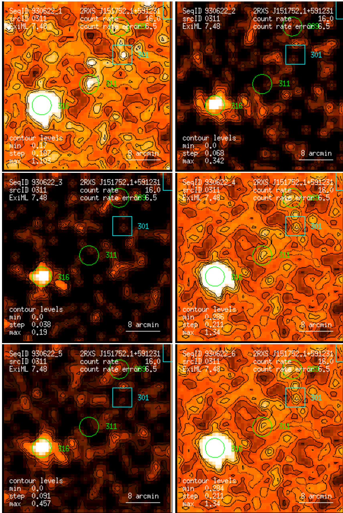
Figure 311: RASS 930622: detection 0311: band rate images, Gaussian filter: (1) PSPC channels 11 – 41, (2) 52 – 90, (3) 91 – 201, (4) 11 – 235, (5) 52 – 201, (6) 11 – 201. Broad band rates in counts/ks. Band rate contour levels in counts/ks/arcmin 2 .
