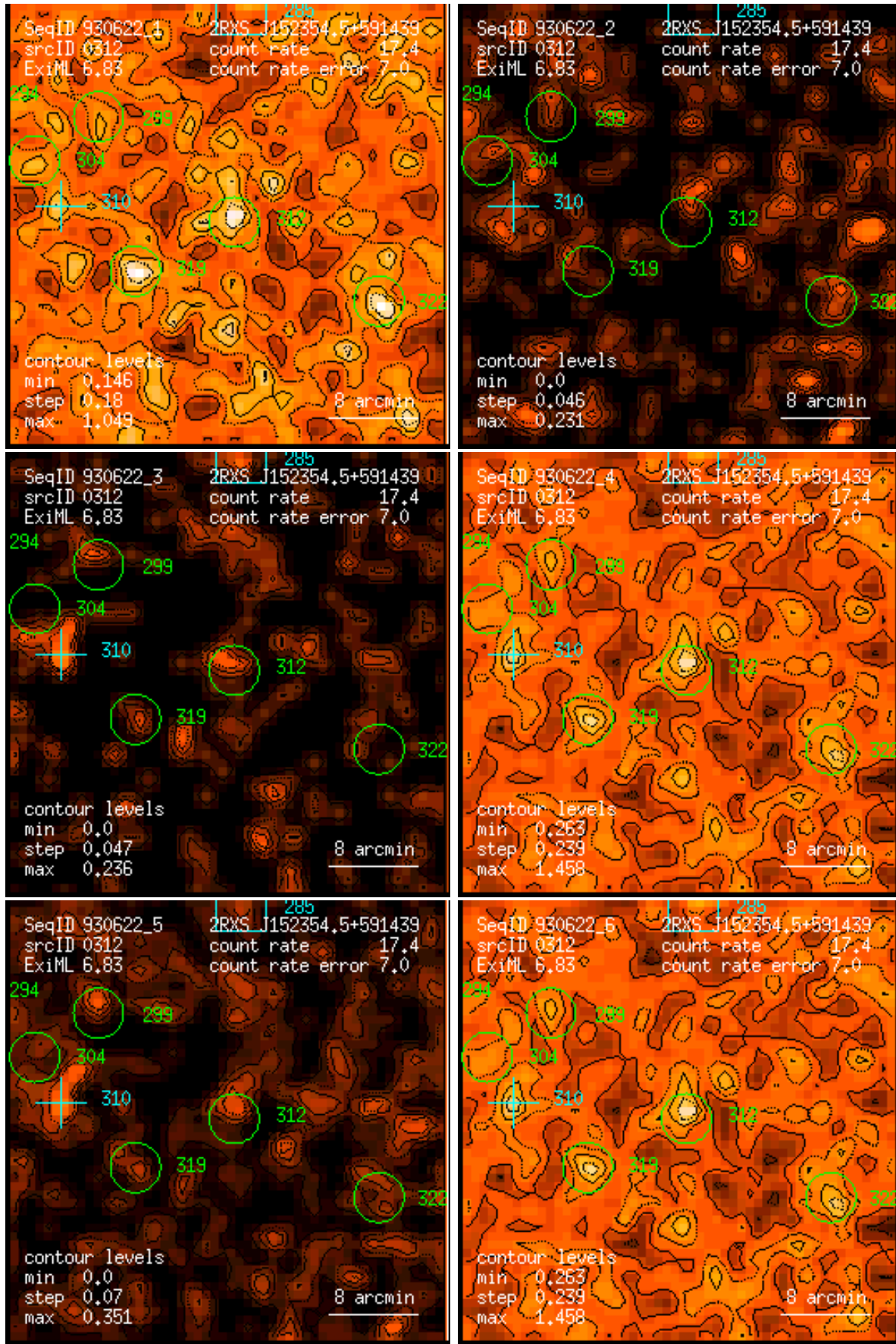
Figure 312: RASS 930622: detection 0312: band rate images, Gaussian filter: (1) PSPC channels 11 – 41, (2) 52 – 90, (3) 91 – 201, (4) 11 – 235, (5) 52 – 201, (6) 11 – 201. Broad band rates in counts/ks. Band rate contour levels in counts/ks/arcmin 2 .
