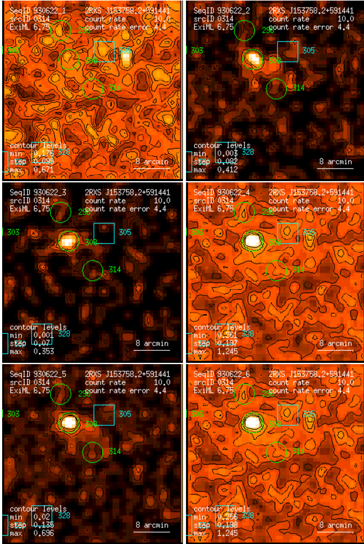
Figure 314: RASS 930622: detection 0314: band rate images, Gaussian filter: (1) PSPC channels 11 – 41, (2) 52 – 90, (3) 91 – 201, (4) 11 – 235, (5) 52 – 201, (6) 11 – 201. Broad band rates in counts/ks. Band rate contour levels in counts/ks/arcmin 2 .
