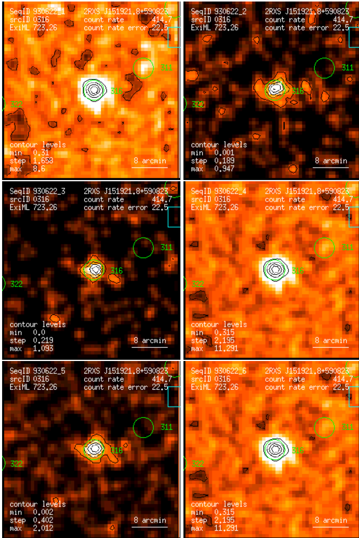
Figure 316: RASS 930622: detection 0316: band rate images, Gaussian filter: (1) PSPC channels 11 – 41, (2) 52 – 90, (3) 91 – 201, (4) 11 – 235, (5) 52 – 201, (6) 11 – 201. Broad band rates in counts/ks. Band rate contour levels in counts/ks/arcmin 2 .
