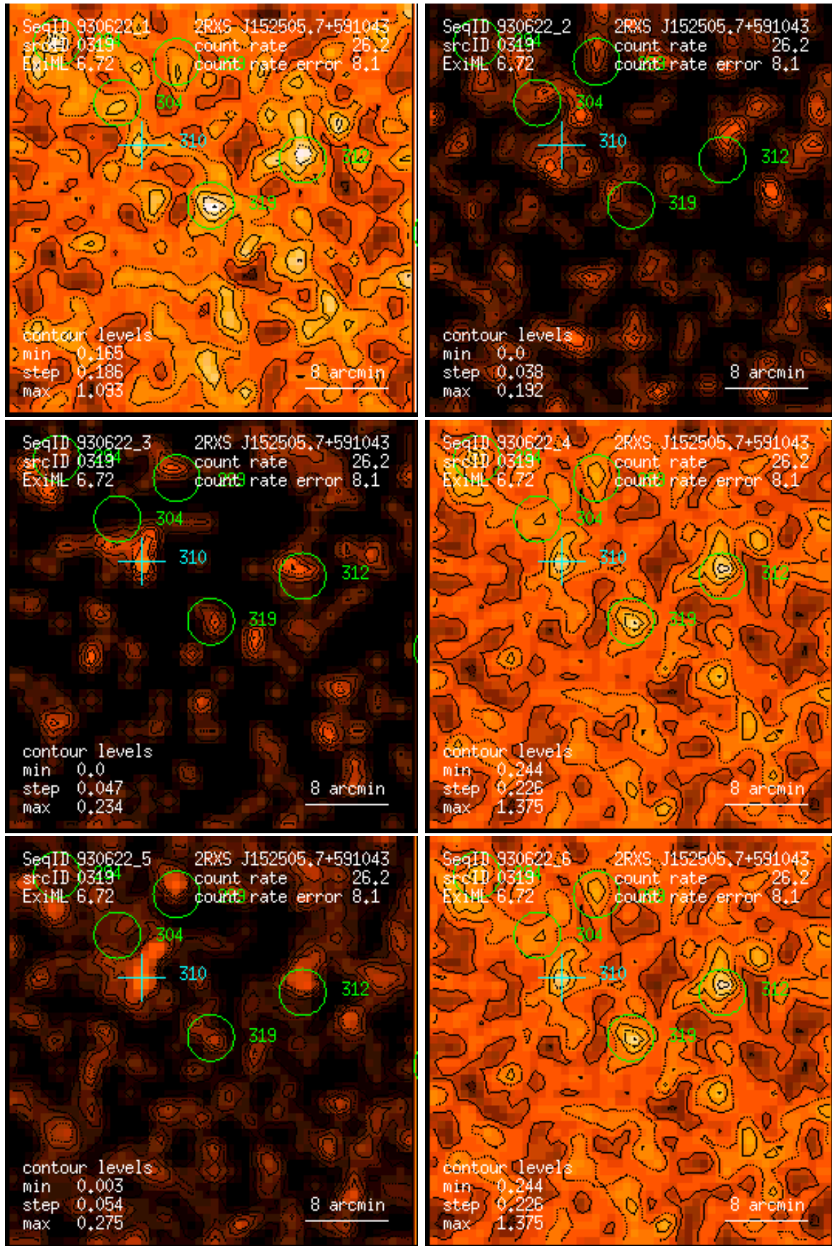
Figure 319: RASS 930622: detection 0319: band rate images, Gaussian filter: (1) PSPC channels 11 – 41, (2) 52 – 90, (3) 91 – 201, (4) 11 – 235, (5) 52 – 201, (6) 11 – 201. Broad band rates in counts/ks. Band rate contour levels in counts/ks/arcmin 2 .
